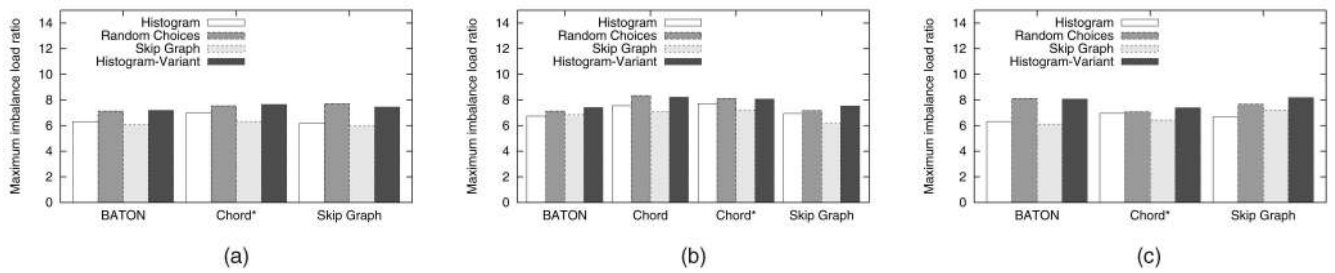
Fig. 14. Maximum load imbalance ratio of nodes. (a) Type-I network (homogeneous nodes, skewed data distribution). (b) Type-II network (heterogeneous nodes, uniform data distribution). (c) Type-III network (heterogeneous nodes, skewed data distribution).
