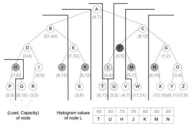
Fig. 8. Histogram structure in BATON.
