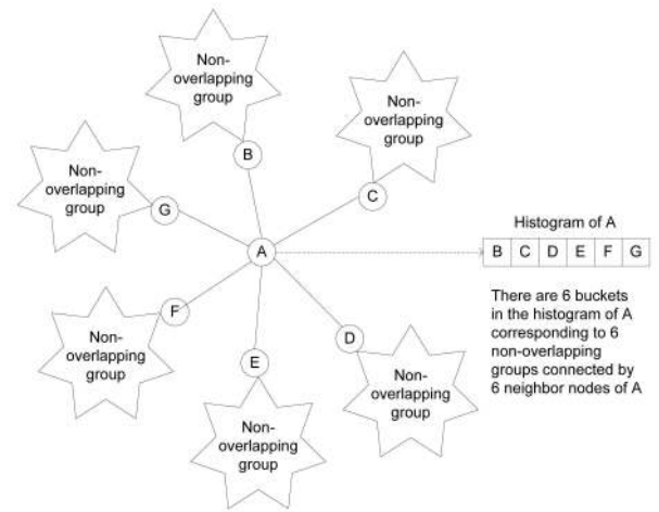
Fig. 1. Histogram structure.
