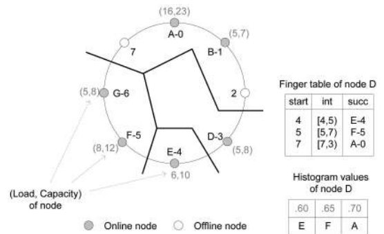
Fig. 10. Histogram structure in Chord.
