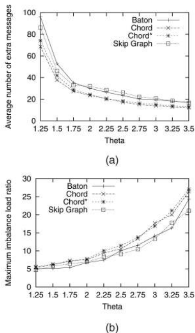
Fig. 16. Effect of varying \theta value in Type-II network (heterogeneous nodes, uniform data distribution). (a) Cost of load balancing. (b) Maximum load imbalance ratio.
