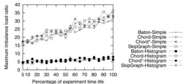
Fig. 13. The change of the maximum load imbalance ratio value along the experiment time line in Type-II network (heterogeneous nodes, uniform data distribution).
