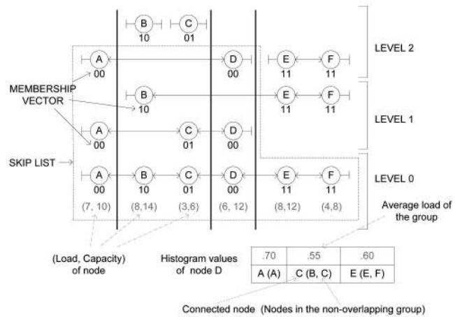
Fig. 5. Histogram structure in Skip Graph.
