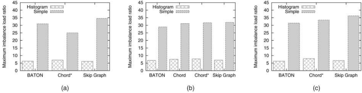
Fig. 12. Maximum load imbalance ratio of nodes. (a) Type-I network (homogeneous nodes, skewed data distribution). (b) Type-I network (homogeneous nodes, skewed data distribution). (c) Type-III network (heterogeneous nodes, skewed data distribution).
