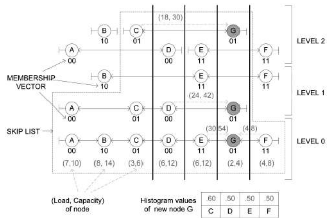
Fig. 6. Histogram construction for a new node in Skip Graph.
