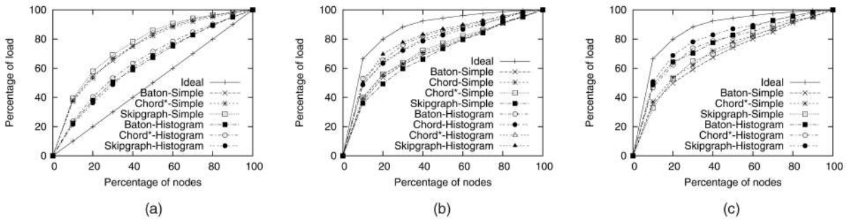
Fig. 11. Load distribution of nodes. (a) Type-I network (homogeneous nodes, skewed data distribution). (b) Type-I network (homogeneous nodes, skewed data distribution). (c) Type-III network (heterogeneous nodes, skewed data distribution).
