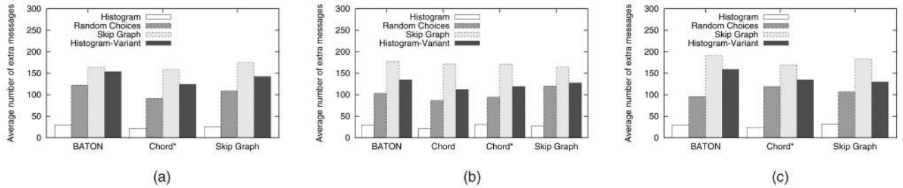
Fig. 15. Cost of load balancing. (a) Type-I network (homogeneous nodes, skewed data distribution). (b) Type-II network (heterogeneous nodes, uniform data distribution). (c) Type-III network (heterogeneous nodes, skewed data distribution).
