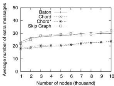
Fig. 17. Effect of varying network size in Type-II network (heterogeneous nodes, uniform data distribution).
