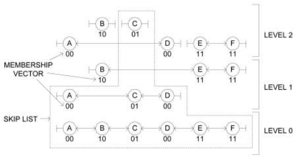
Fig. 4. A skip graph with three levels.
