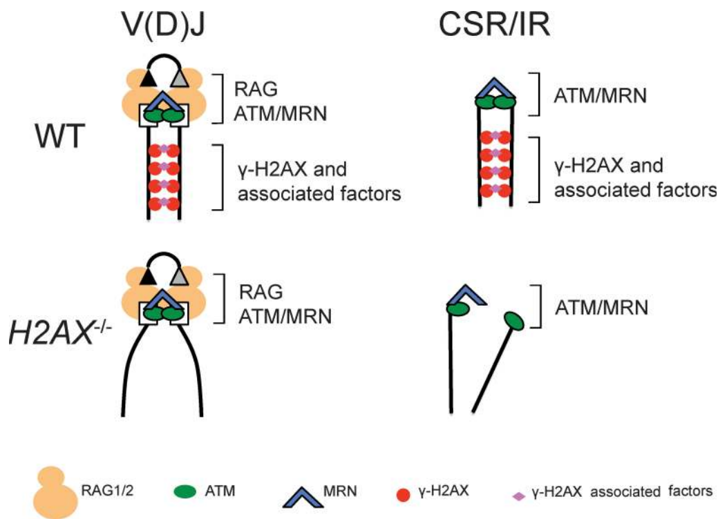
Figure 6. Models of H2AX function during end-joining repair of chromosomal DSBs. Schematic diagrams depicting the potential positional stability of broken chromosomal DNA strands during V(D)J recombination, CSR, or general DSB repair in G1-phase wild-type and H2AX-deficient cells. Boxes and triangle represent RAG-generated coding and signal ends, respectively. H2AX-mediated stabilization of broken DNA strands would be dispensable for end joining during V(D)J recombination as a result of DNA end stabilization by ATM/MRN and RAG postcleavage synaptic complexes. However, this H2AX function would be important for end joining during CSR and general DSB repair.
