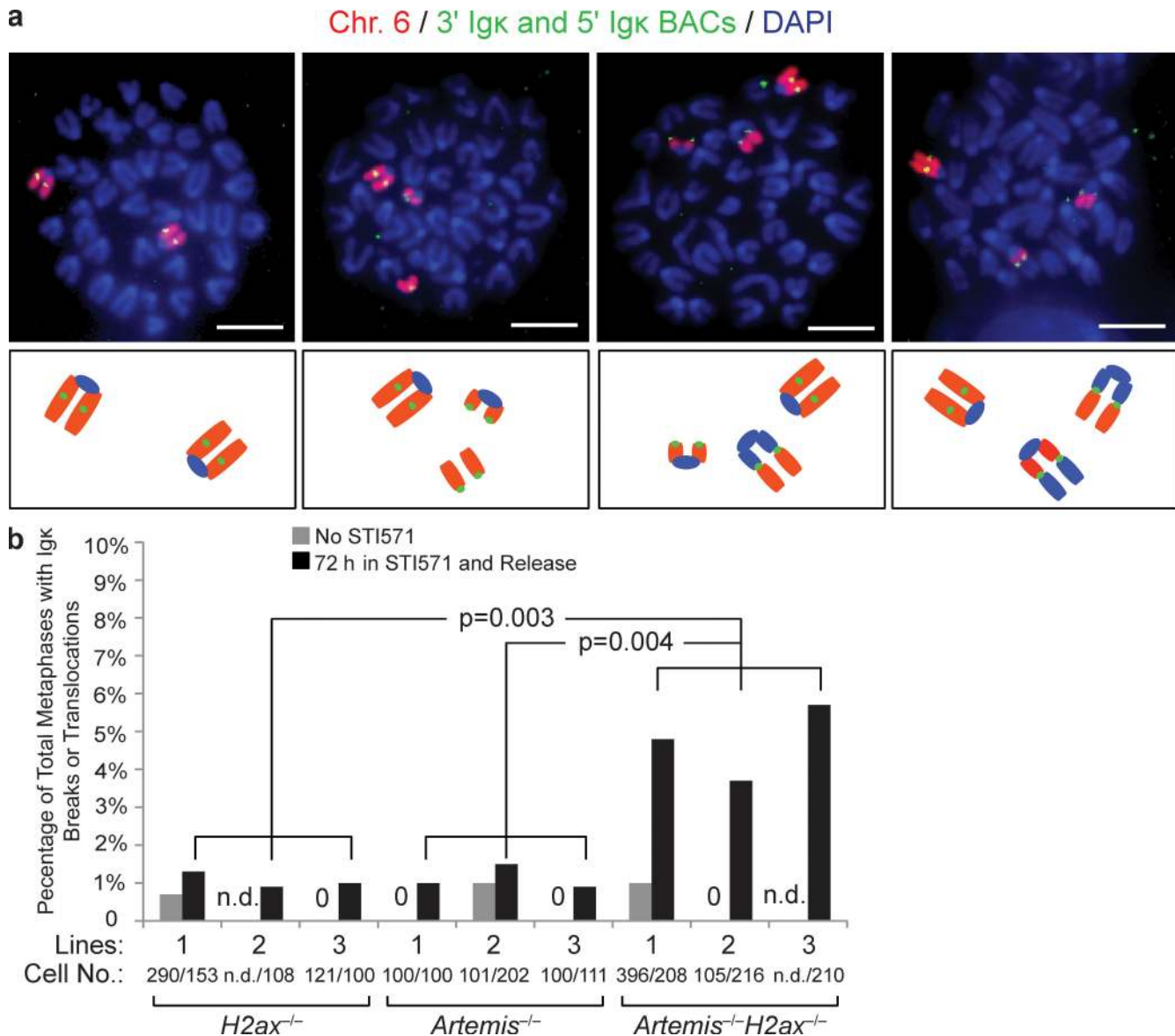
Figure 4. H2AX prevents transition of RAG-cleaved Igk DNA strands into chromosome breaks and translocations during cellular proliferation. (a) Shown are representative fluorescent light microscopy images of whole chromosome (Chr.) 6 paints (red) and FISH analysis using the 5' V \kappa and 3' C \kappa BACs (both green) and DAPI (blue) to visualize DNA on metaphases prepared from STI571-treated and released Artemis -/- H2ax -/- abl pre-B cells. Below each image is a schematic representation of the observed chromosome 6 configurations. Images show from left to right: two intact chromosome 6; an intact chromosome 6 and a chromosome 6 with an Igk locus break; an intact chromosome 6 and a chromosome 6 broken into two fragments with one resolved as an Igk locus translocation; and an intact chromosome 6 and a broken chromosome 6 that resolved as two distinct Igk locus translocations. Bars, ~1 \mu m. (b) Shown is a bar graph with quantification of RAG-initiated Igk chromosome breaks or translocations in metaphases prepared from cells of three independent H2ax -/- , Artemis -/- , and Artemis -/- H2ax -/- pre-B cell lines released from STI571 treatment. Metaphases prepared from cells of the same lines without STI571 treatment were assayed for Igk chromosome breaks or translocations to control for potential spontaneous rearrangement and genomic instability accumulated during cell culture. The data represents the percentage of total metaphases analyzed that contained Igk chromosome abnormalities. The numbers of metaphases assayed to generate the representative data are indicated. 0, Igk abnormalities were not observed; n.d., not determined. The p-values for comparison between cells of the indicated different genotypes are shown. These data were obtained from the same experiment performed three independent times.
