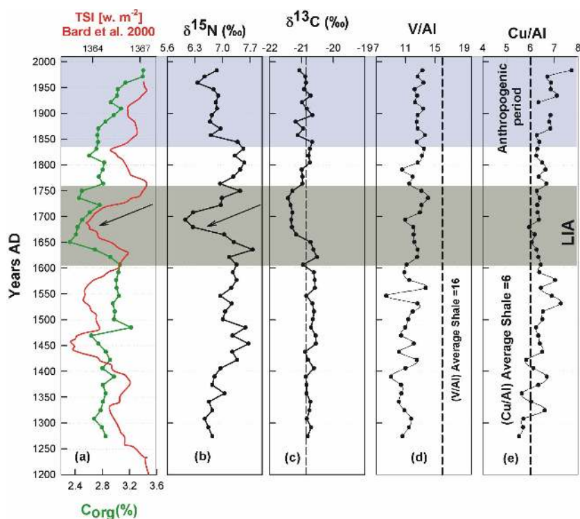
Fig. 15. Profiles of selected productivity and redox proxies in the Gravity Core CR-2 from the inner shelf region off Goa (Lat. 14.80° N, Long. 74.20° E; water depth ~45 m) in the eastern Arabian Sea. (a) Total solar irradiance (TSI) from Bard et al. (2000) and organic carbon (Corg). (b) \delta^{15}\text{N} of sedimentary organic matter, (c) \delta^{13}\text{C} of Corg, (d) V/Al and (e) Cu/Al. The core was dated by C-14 and Pb-210 techniques. The arrows within the grey portion point to the Maunder Minimum of the Little Ice Age (LIA) whereas the upper portion of the core corresponding to the Anthropocene period is shown in purple (modified from Agnihotri et al., 2008).
