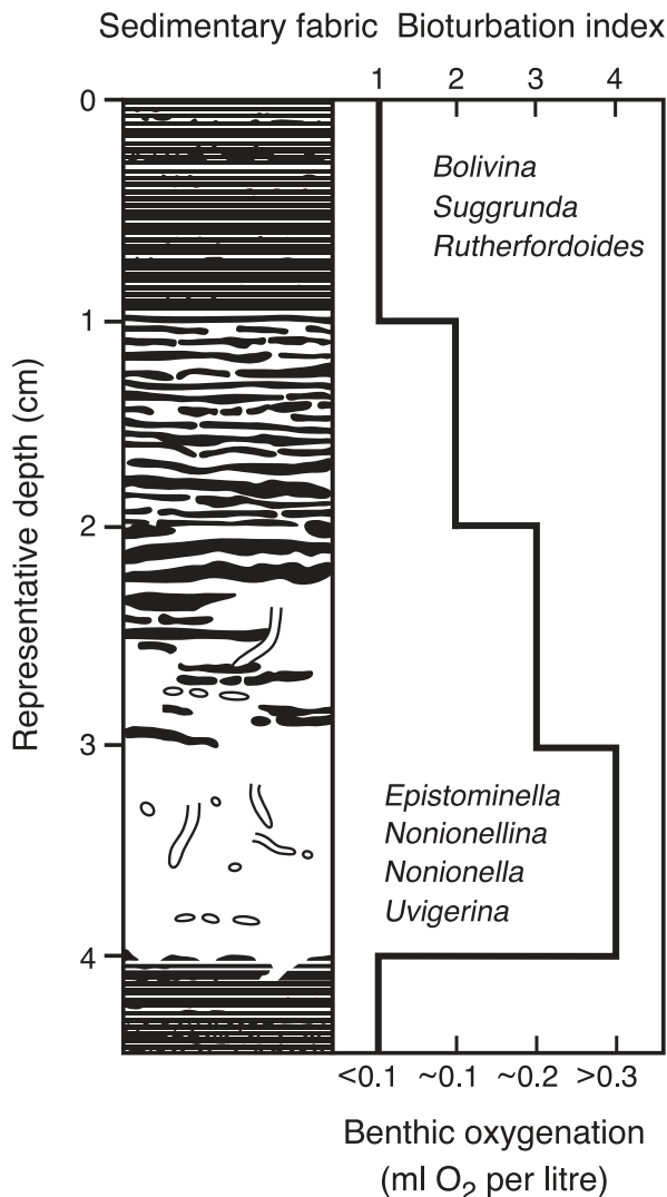
Fig. 18. Bioturbation index (BI) based on the development of sediment laminations; application to sediments from Santa Barbara Basin (576-m water depth), NE Pacific. BI value 1 = sediments with distinct, continuous laminations. BI value 2 = diffuse, discontinuous irregular laminations. BI value 3 = slightly bioturbated with either faint, diffuse laminations or a few discrete patches of laminations surrounded by homogenized sediment, including local Chondrites burrows. BI value 4 = completely bioturbated, fine-grained sediments with no discernable fabric and commonly containing echinoid spines. Characteristic foraminiferans are listed for two end-member facies. The four facies recognized are believed to correspond approximately to the following oxygen concentrations: <0.1 \text{ mL L}^{-1} ( <4.3 \mu\text{M} ; facies 1), macrofauna excluded; 0.1 \text{ mL L}^{-1} ( 4.3 \mu\text{M} ; facies 2), meiofaunal bioturbation causing laminations to become diffuse; 0.1\text{--}0.2 \text{ mL L}^{-1} ( 4.3\text{--}8.6 \mu\text{M} ; facies 3), enough oxygen to permit partial homogenization of sediment by fauna; >0.3 \text{ mL L}^{-1} ( >13 \mu\text{M} ; facies 4), macrofauna present. Reprinted from Behl and Kennett, 1996, with permission from Macmillan Publishers Ltd (Nature).
