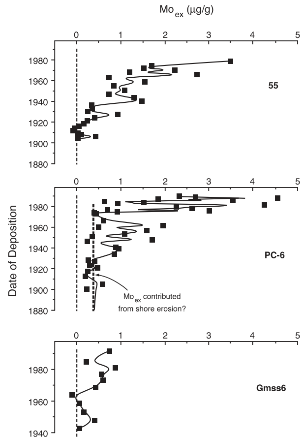
Fig. 10. Excess molybdenum concentration ( \text{Mo}_{\text{ex}} ) in three cores from the middle and upper part of Chesapeake Bay. The heavy dotted line in the central panel suggests a baseline input of \text{Mo}_{\text{ex}} from shore erosion. The curve shows the gross trends in the data, suggesting increasingly intense seasonal oxygen depletion. (Redrawn from Geochimica et Cosmochimica Acta , Vol. 65, Adelson, J. M., Helz, G. R., and Miller, C. V.: Reconstructing the rise of coastal anoxia: molybdenum in Chesapeake Bay sediments, 237–252, 2001, with permission from Elsevier.)
