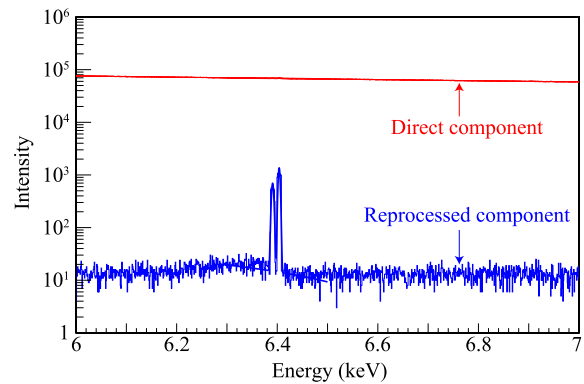
Fig. 8. The Monte Carlo simulation result using MONACO. Red shows the direct X-ray continuum, while blue represents a reprocessed emission including Fe-K \alpha_1 and Fe-K \alpha_2 lines. (Color online)
