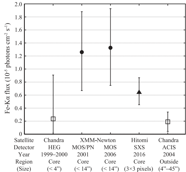
Fig. 4. Comparison of the Fe-K \alpha fluxes among different satellites, instruments, years, and regions. Open squares, filled circles, and filled triangle show the Fe-K \alpha fluxes obtained by Chandra, XMM-Newton, and Hitomi, respectively. Error bars show 90% confidence ranges.
