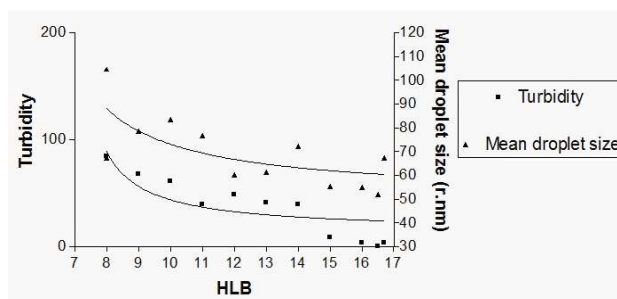
Figure 5. Curves of mean droplet diameter and turbidity of Rosmarinus officinalis emulsions versus HLB (ANOVA, p < 0.05 ).
