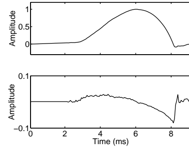
Fig. 6. Example of a library pulse and its time derivative. The pulse is extracted from a sustained vowel [a] produced by a male speaker using normal phonation. The closed phase of the original pulse derivative was forced to zero in order to remove minor fluctuations present in the waveform produced by the glottal inverse filtering.
