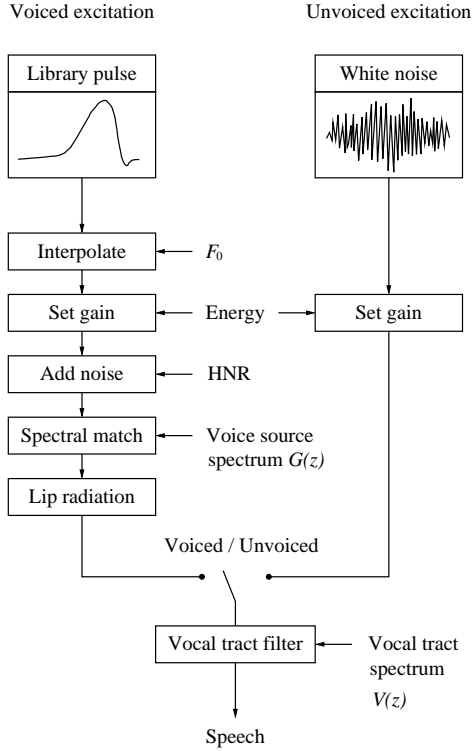
Fig. 7. Flow chart of the synthesis stage. The basis of the voiced excitation signal is a library glottal flow pulse, which is modified according to the voice source parameters. Unvoiced excitation is composed of white noise. The excitation signals are combined and filtered with the vocal tract filter V(z) to generate speech.
