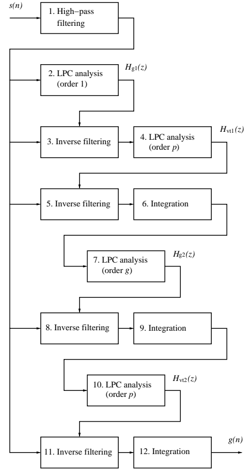
Fig. 2. Block diagram of the IAIF method. The glottal flow signal g(n) is estimated through an repetitive procedure of canceling the effects of the vocal tract and the lip radiation from the speech signal s(n) .
