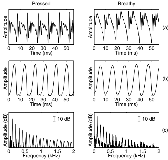
Fig. 1. (a) Waveform of a sustained vowel [a] produced by a male speaker using pressed (left panel) and breathy (right panel) phonation. (b) Corresponding glottal flow signals estimated with the iterative adaptive inverse filtering (IAIF) method [24], [32]. In pressed phonation (left), the glottal flow pulses are shorter compared to breathy phonation and there is a clear closed phase between the pulses. (c) Spectra of the estimated glottal flow signals (only shown for 0–2 kHz). The spectrum of the breathy phonation (right) shows a clear emphasis on the fundamental frequency component. The spectral envelope is also steeper and there is more noise at the higher frequencies.
