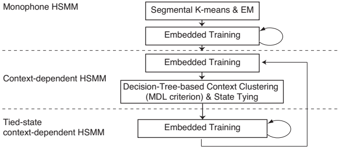
Fig. 5. Overview of the training stages of HMMs. First, monophone HSMs are trained, converted into context-dependent HSMs, and re-estimated. Then, decision-tree-based context clustering is applied to the HSMs and the model parameters of the HSMs are tied. Finally, the clustered HSMs are re-estimated again.
