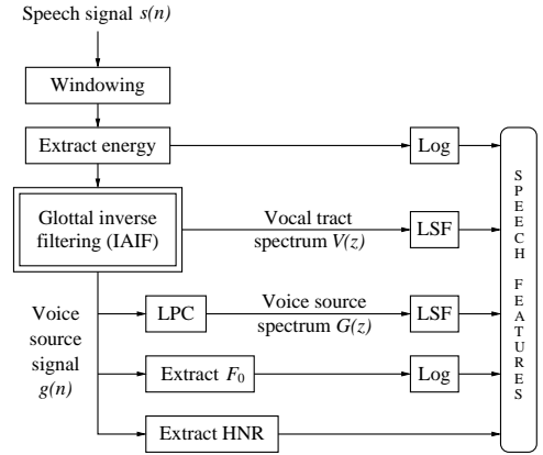
Fig. 4. Flow chart of the parametrization stage. The speech signal s(n) is decomposed into the glottal source signal g(n) and the all-pole model of the vocal tract V(z) using the IAIF method. The glottal source signal is further parametrized into the all-pole model of the voice source G(z) , the fundamental frequency F_0 , and the harmonic-to-noise ratio (HNR). The obtained parameters are converted to a suitable representation for the HMM system. For clarity, the parametrization of unvoiced speech segments, using basic LPC for the estimation of spectrum, is excluded from the flow chart.
