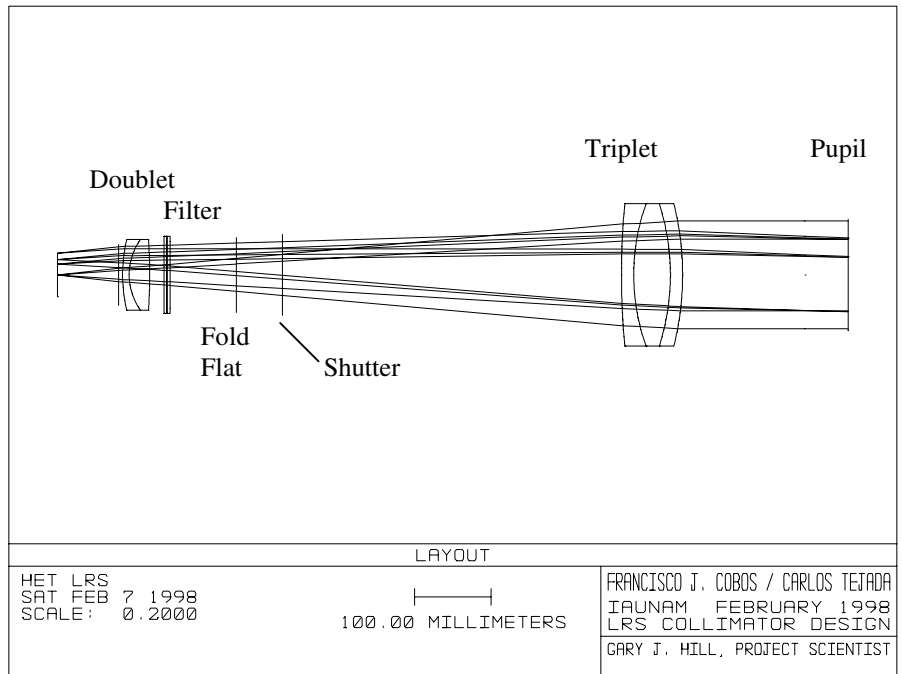
Figure 1. Layout of the LRS collimator
