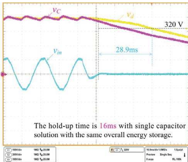
Figure 9. Hold-up time of the dc-link module in a 390 V dc-link PFC power converter ( C : 450 V/110 \mu F, C_c : 63 V/940 \mu F, 170 W load testing, v_c : 100 V/div, v_d : 100 V/div, v_{in} : 300 V/div and timescale: 10ms/div).
