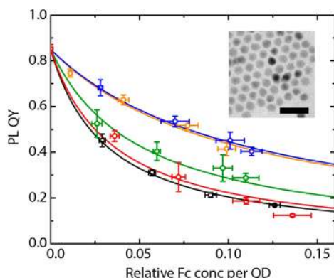
Figure 4. Photoluminescence quantum yield (PLQY) of QD sample 1 as a function of the relative concentration of ferrocene ligand bound to the surface. Fits to eq 1 are shown as solid lines. \text{Br}_3\text{FcOC}_6\text{SH} (orange), \text{Br}_2\text{FcOC}_6\text{SH} (blue), \text{BrFcOC}_6\text{SH} (green), \text{FcOC}_6\text{SH} (red), and \text{FcC}_6\text{SH} (black) were exchanged onto this sample. Inset: TEM micrograph of QD sample 1 with 25 nm scale bar.
