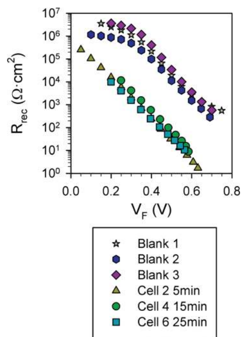
Figure 5. Recombination resistance, R_{rec} , under dark conditions for different applied voltages for different TiO_2/Sb_2S_3/CuSCN solar cells (with different CuSCN deposition times) and for blank TiO_2/CuSCN cells, calculated from the fitting of the impedance spectra.
