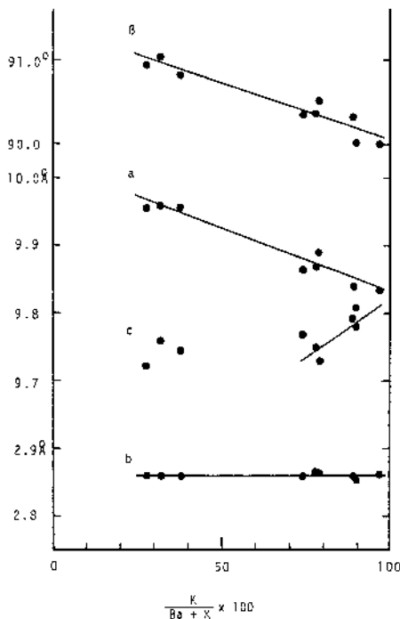
FIG. 4. Relation between cell dimensions and K/(K+Ba) of hollandite and cryptomelane from Tirodi mine.
