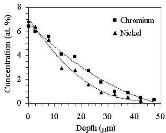
Figure 7. Cr and Ni concentration profiles for a sample submitted to a previous deposition treatment following on the hollow cathode discharge sintering experiment.
