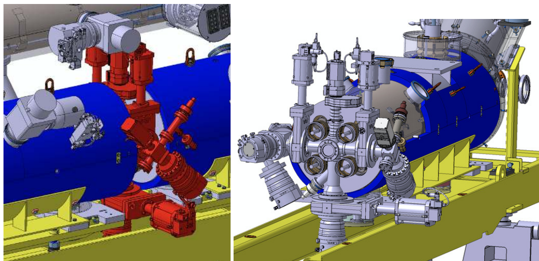
Figure 14. Preliminary design of the BGC monitors installed in the middle of the HEL, between the two main solenoids, to measure at the same time 2D profiles of the proton and electron beams: 3D view showing the integration between the magnet cryostat (left) and cut view of the transverse cross section (right). Courtesy of I. Papazoglou and G. Schneider, CERN, SY-BI.
