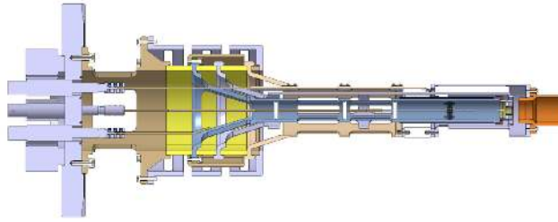
Figure 11. Cross section of the HL-LHC thermionic gun, optimized for the small cathode design with outer radius of 8.05 mm, from [37].
