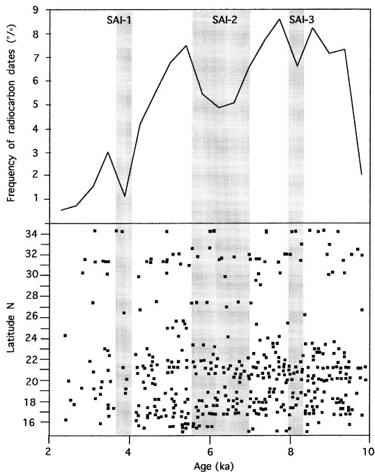
Fig. 1. Temporal and latitudinal distribution of the surface fresh water indicators from the Sahara. (a) Age frequency of the radiocarbon dated markers. The frequencies are calculated at 400-year intervals and expressed as a percentage of the total number (560 dates). The drier episodes are marked by shaded zones. (b) Latitudinal distribution of the dated markers.
