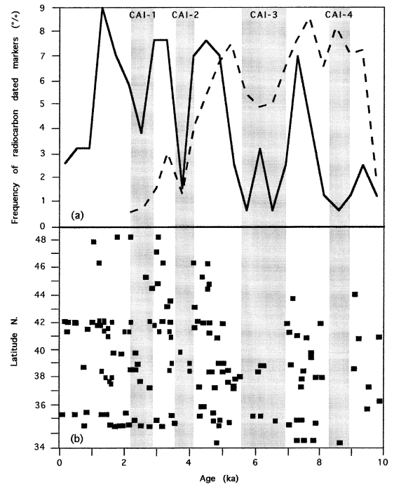
Fig. 2. Temporal and latitudinal distribution of humid indicators (palaeosols and lacustrine sediments) from the deserts in northern China. (a) Age frequency of the radiocarbon dated markers (continuous line) compared with that of the Sahara (dotted line). The frequencies are calculated at 400-year intervals and expressed as a percentage of the total number (158 dates). The drier episodes are marked by shaded zones. (b) Latitudinal distribution of the dated markers.
