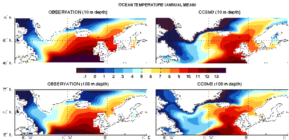
Fig. 3. Comparison of the mean annual temperature at 10 m and 100 m between CCSM3 and WOA98. NODC WOA98 data were provided by the NOAA/OAR/ESRL PSD, Boulder, Colorado, USA, from their Web site at http://www.esrl.noaa.gov/psd/ .
