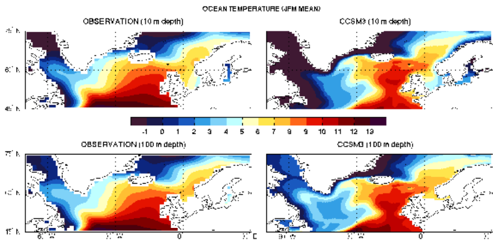
Fig. 4. Comparison of the mean January, February, and March temperature at 10 m and 100 m between CCSM3 and WOA98. NODC WOA98 data were provided by the NOAA/OAR/ESRL PSD, Boulder, Colorado, USA, from their Web site at http://www.esrl.noaa.gov/psd/ .
