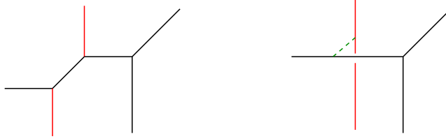
Figure 21: Web diagram for the SPP and its deformation to a smooth geometry.
