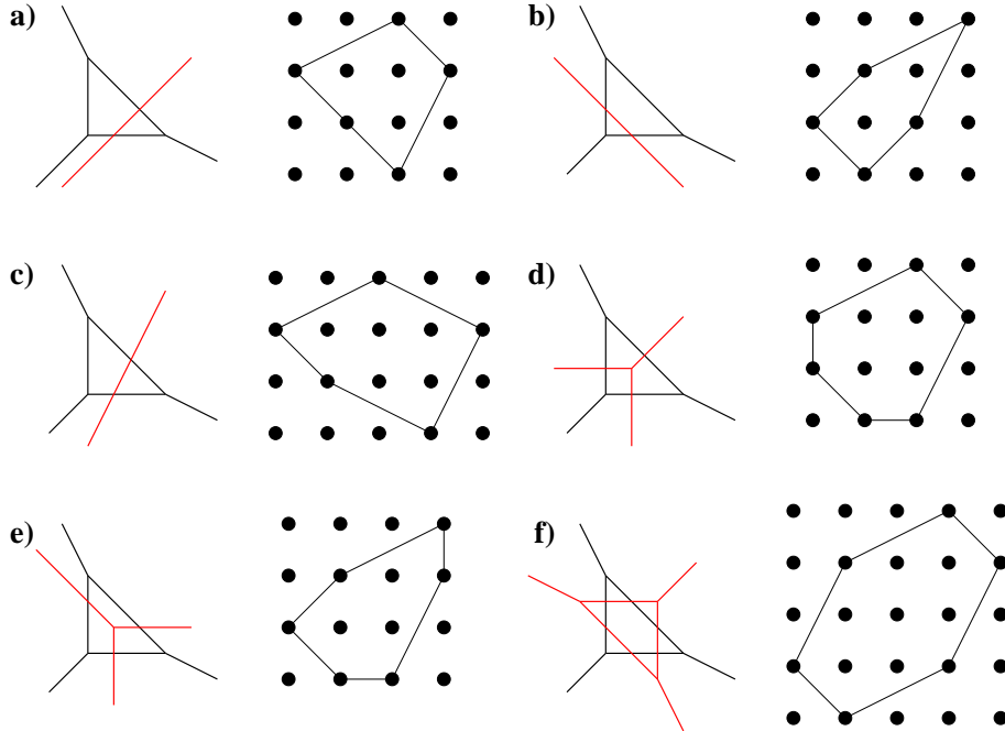
Figure 4: Web and toric diagrams for diverse examples of geometries Y which admit a complex deformation to the \mathbf{C}^3/\mathbf{Z}_3 singularity. The web diagrams are shown at the origin of the deformation branch, and the subwebs to be removed is shown in red.
