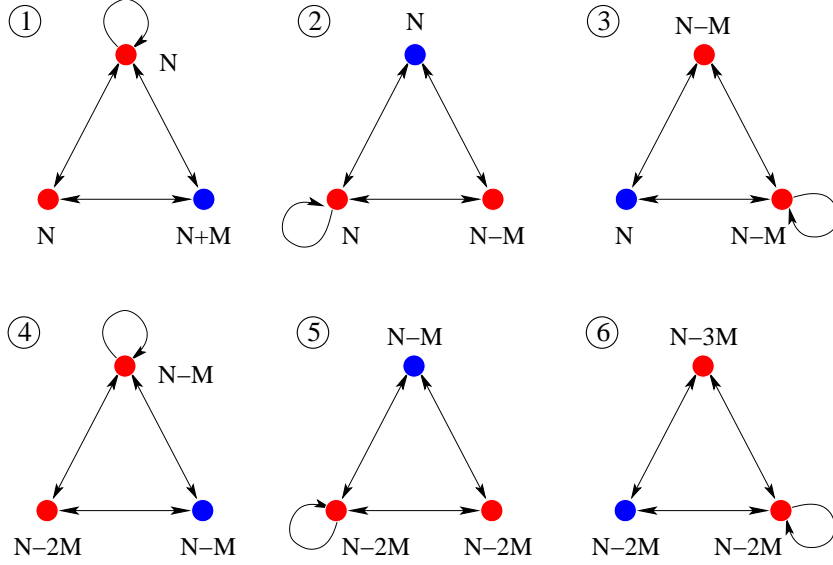
Figure 20: Sequence of quivers in one period of the SPP cascade. We have indicated in blue the dualised node at each step.
