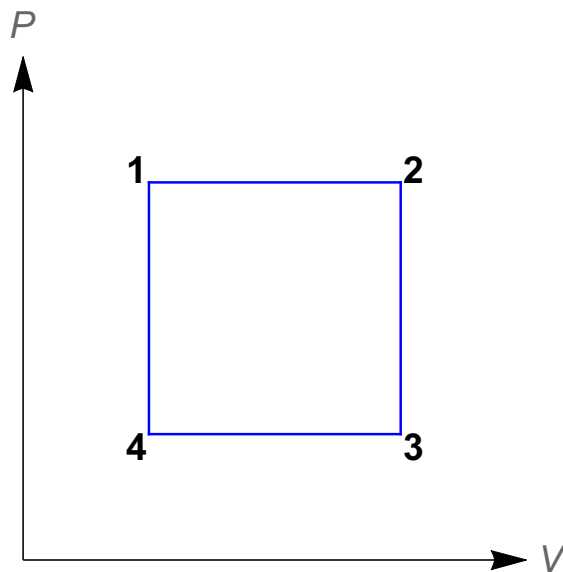
Figure 8. The isobar-isochore engine. The vertical lines are isochores, and the horizontal lines are isobars. In terms of the boundary theory, an isochore can be interpreted as a process where N is varied while keeping the cutoff \Lambda_c^* fixed. In an isobar process, on the other hand, \Lambda_c^* is varied while N is kept fixed.
