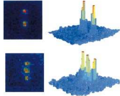
Fig. 7. Fluorescent images for two-trap and three-trap arrays, showing control of the zeroth order. The two traps in the top figures were generated symmetrically with respect to the zeroth-order diffraction spot; the middle trap in the bottom figure was generated from the zeroth order.
