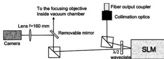
Fig. 4. Experimental setup for phase modulation of the dipole trap beam. The removable mirror placed in the beam path is used to send light to an imaging camera that records the geometry and shape of the generated pattern.
