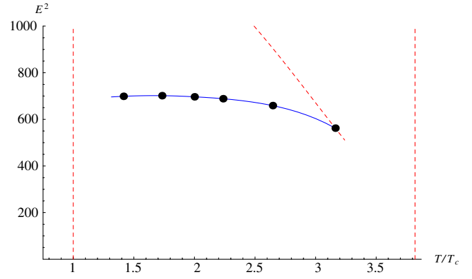
FIG. 12 (color online). Analysis of the temperature dependence of the energy of U -shaped strings. Displayed are the squared energies of a state of spin J \approx 1.5 , which dissociates at T/T_c = 3.16 when L/R = 0.24 . The diagonal dotted curve shows the maximum possible energy for a given temperature. Note the qualitative similarity with the low-spin plot, Fig. 5.
