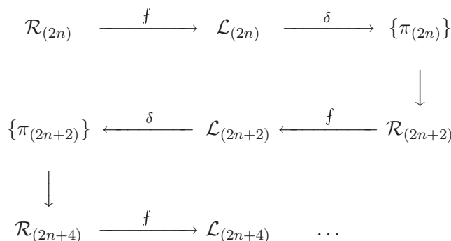
Figure 1. A schematic illustration of the algorithm used to determine Hamilton's principal function iteratively. Here, the operators f and \delta stand respectively for the functional integration defined by the formula in (2.38) and for functional differentiation with respect to the induced fields.
