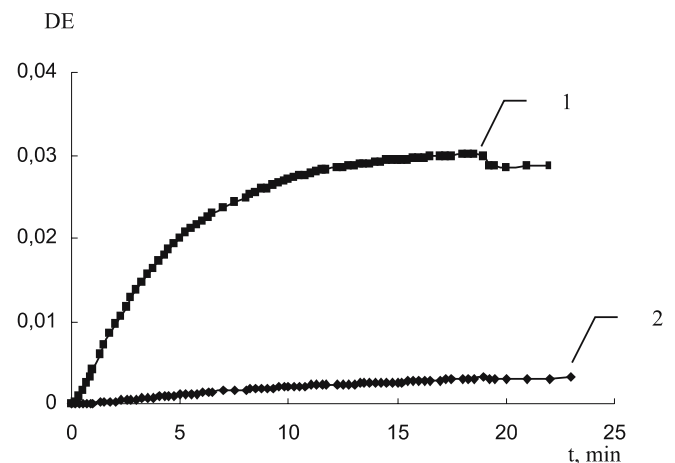
FIGURE 2 The diffraction efficiency kinetics of the first (1) and the second (2) orders during exposure (4 mol.% PQ, h = 85\ \mu\text{m} , d = 1.65\ \mu\text{m} )
