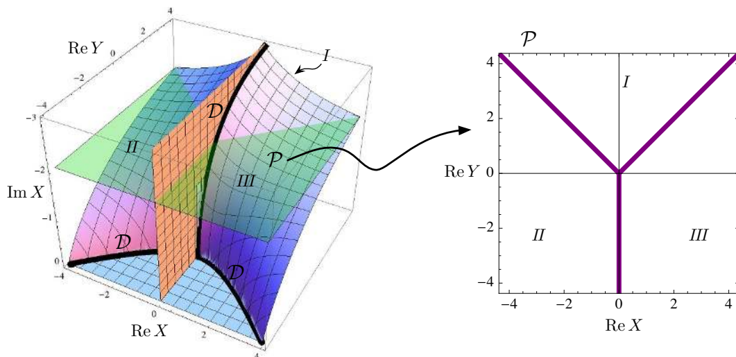
Figure 19. Some Stokes walls for the \mathbb{CP}^1 sigma-model at \text{Im } Y = 0 , emanating from the discriminant locus \mathcal{D} . The plane \mathcal{P} at \text{Im } X = -2\pi/3 , highlighted in green on the left, is reproduced on the right.
