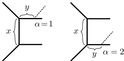
Figure 21. Toric geometry for T_1 .
