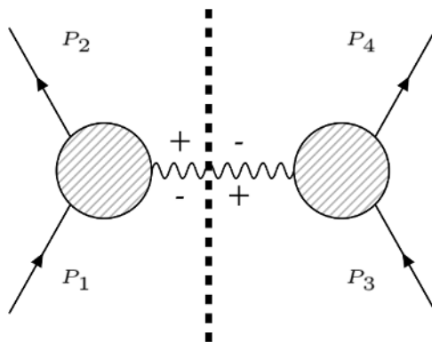
Figure 2. A one photon/graviton exchange process. In the HCL the internal particle is on-shell and the two polarizations need to be considered.
