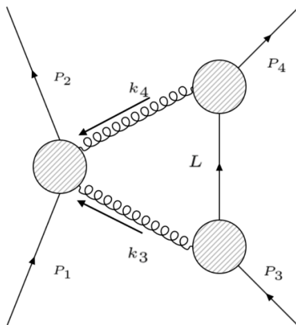
Figure 3. The triangle diagram used to compute the leading singularity, corresponding to the b -topology. The a -topology is obtained by reflection, i.e. by appropriately exchanging the external particles.
