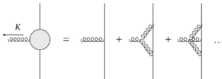
Figure 4. The matrix element of the stress-energy tensor \langle T_{\mu\nu}(K) \rangle corresponds to the 3 point function associated to a pair of massive particles and an external off-shell graviton. The coupling to internal gravitons emanating from the massive source yields, in the long-range behavior, higher corrections in G .
