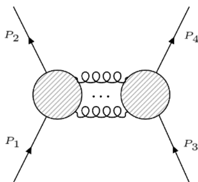
Figure 1. A typical scattering process contributing to the effective potential. In this case two massive particles represented by P_1^2 = P_2^2 = m_a^2 and P_3^2 = P_4^2 = m_b^2 exchange several gravitons. The momentum transfer is given by K = P_1 - P_2 = (0, \vec{q}) in the COM frame.
