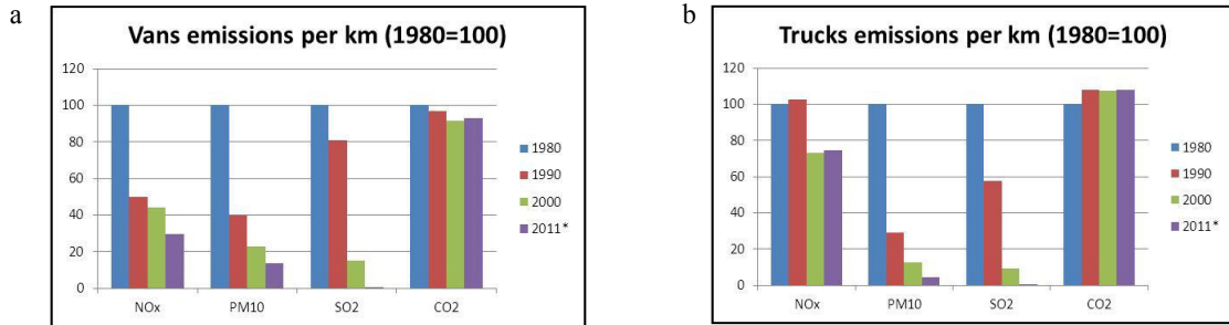
Fig. 5. (a) Vans and (b) trucks emissions of NO x , PM10 and CO 2 between 1980 and 2011 [indexed, per km] (Source: Moorman & Kansen, 2011)
