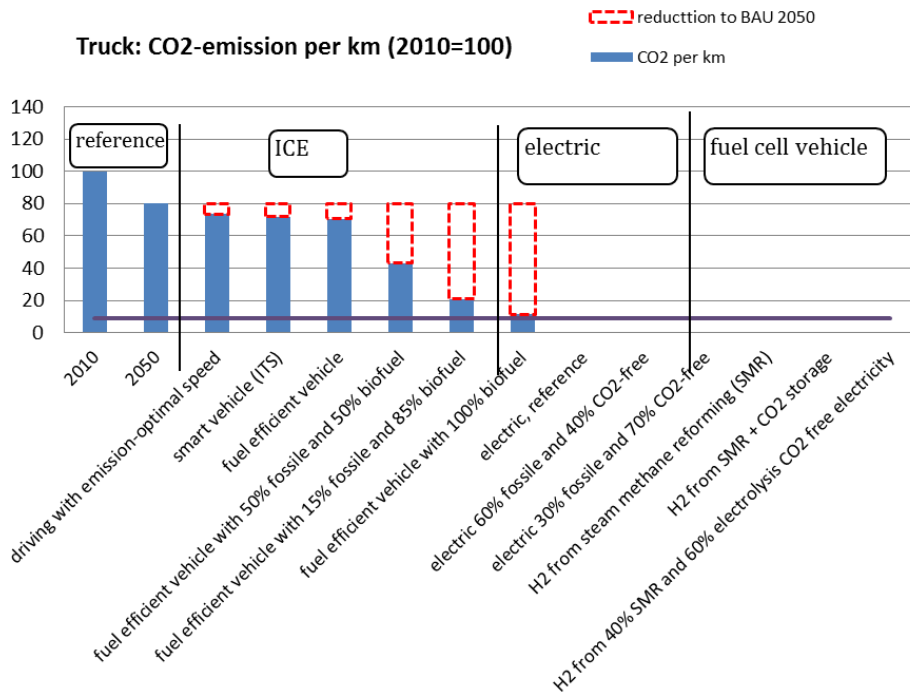
Fig. 7. CO 2 emission per km for trucks in 2050 with different technologies (Source: Moorman & Kansen, 2011)
