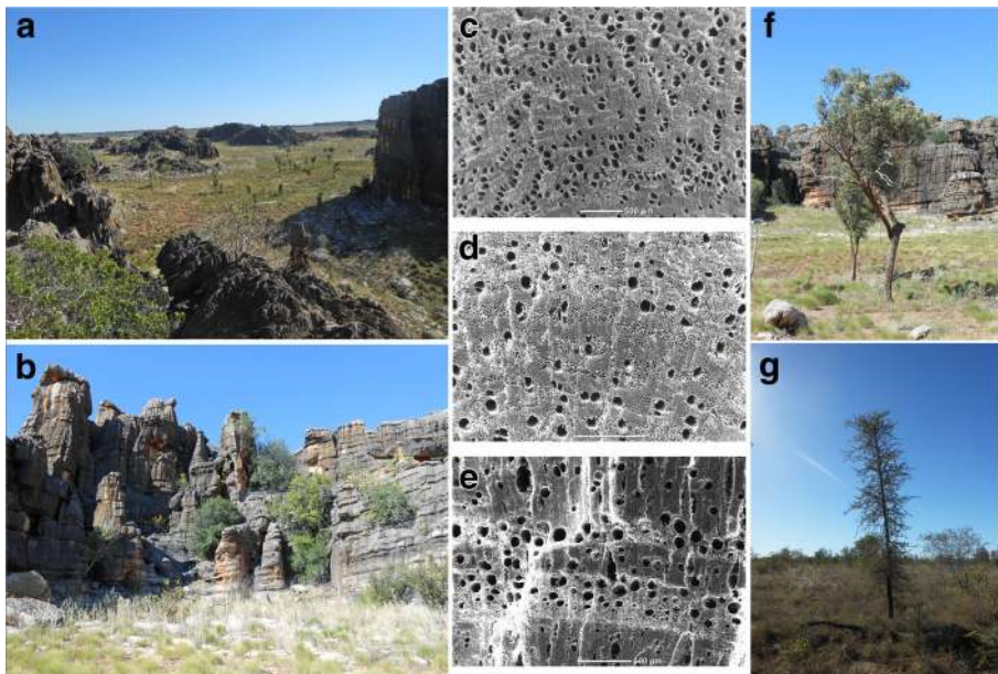
Fig. 11 Vegetation types and their common charcoals. Left, low tree steppe of the Riwi valley floor (a), dry rainforest taxa colonise the limestone outcrop (b); centre, reference SEM images of Corymbia dampieri (c), Vachellia suberosa (d), Brucea javanica ; right: Corymbia sp. (f) and Vachellia suberosa (g) (photos and SEM by R. Whitau)
