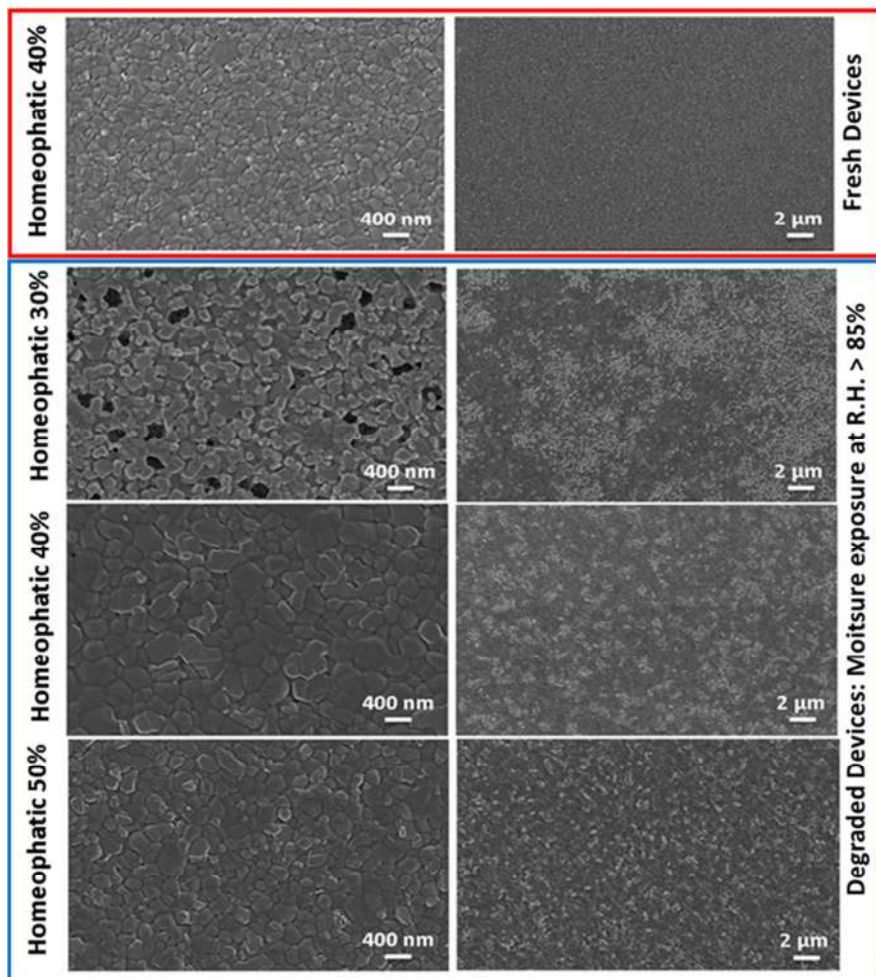
38 39 Figure 2. SEM images of fresh perovskite films fabricated at R.H.=40% (top) and after degradation 40 (bottom). Results for degraded films with very humid air (> 85% R.H.) but prepared at different ambient 41 humidity values are shown. 42 43 44
