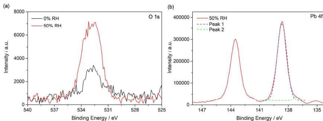
34 35 36 37 38 39 40 41 42 43 44 45 46 47 48 Figure 3. O 1s and Pb 4f signals obtained from XPS measurements of perovskite thin films deposited on 49 top of mesoporous TiO 2 layers fabricated at different ambient humidity values. 50 51 52
