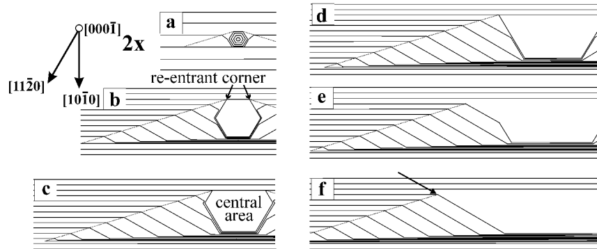
Figure 3. Schematic representation of the time-dependent development and subsequent overgrowth of a hexagonal hillock. Image a) is two times enlarged. The arrow in f) indicates the discontinuity line on the plateau, cf. figure 2c.
