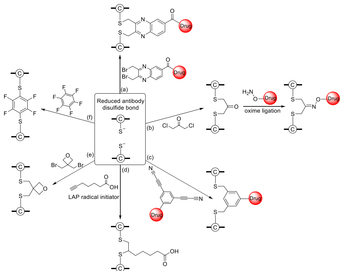
Scheme 4 – Other reagents employed for disulfide bridging on antibodies or antibody fragments; a. C-Lock™ technology employing dibromomethyl heterocyclic aromatic groups, b. dichloroacetone, followed by oxime ligation, c. arylenedipropionitrile (ADPN), d. thiol-yne coupling with 6-heptynoic acid, e. 3,3-bis(bromomethyl) oxetane, f. hexafluorobenzene.
