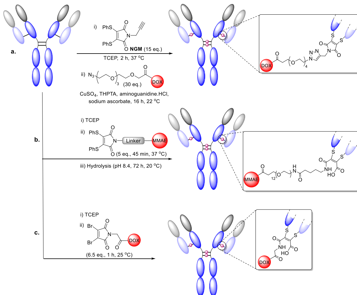
Scheme 2 – ADC construction by disulfide bridging using next-generation maleimides; a. dithiophenol-maleimide with alkyne handle, b. dithiophenolmaleimide attached to MMAE through a non-cleavable C6-PEG 12 spacer, c. optimized DAR 4 ADC preparation using a dibromomaleimide containing a C2 spacer, linked to doxorubicin.
