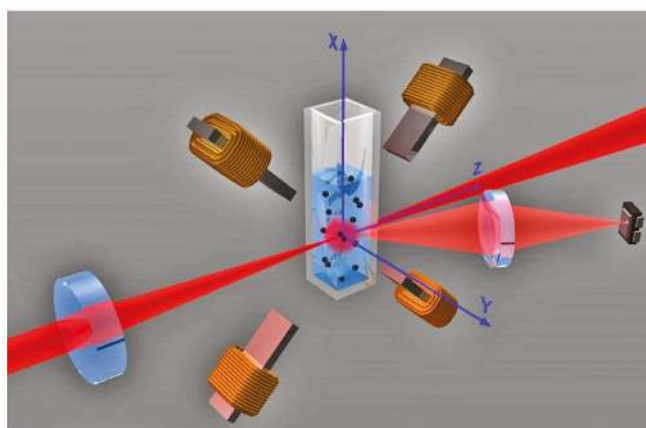
Figure 11. Sketch of the setup for analyte detection by scattering observation of the magnetorotation of magnetic particle label clusters. Reprinted with permission from [232]. Copyright 2011, American Chemical Society.
