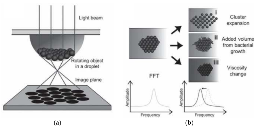
Figure 12. Sketch of the bead assembly magnetorotation detection principle. (a) At the bottom of a hanging droplet, a cluster of magnetic particles forms, and the response of the cluster to an applied rotating magnetic field is observed optically in the imaging plane; (b) Changes in cluster assembly (particle density or total cluster volume) or variations in local fluid viscosity lead to an altered rotation frequency of the cluster, which is analyzed from the optical signal by fast Fourier transformation (FFT). Reprinted with permission from [235]. Copyright 2012, John Wiley and Sons.
