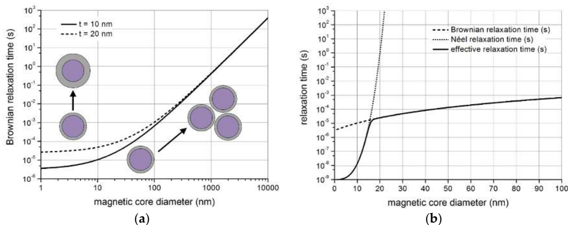
Figure 3. Brownian, Néel and effective relaxation time in dependence of the particle volume. A spherical magnetite particle with a magnetic core (purple area) encapsulated by a hydrodynamic shell (grey area) of thickness t is assumed: (a) Brownian relaxation time in dependence of the magnetic particle core diameter for hydrodynamic shell thicknesses of 10 nm (solid line) and 20 nm (dashed line). While an increase of the hydrodynamic shell thickness affects the Brownian relaxation time of small particles at short relaxation times, particle clustering induces large changes of the relaxation time less dependent of the initial particle size; (b) Brownian, Néel and effective relaxation time as functions of the magnetic core diameter [112].
