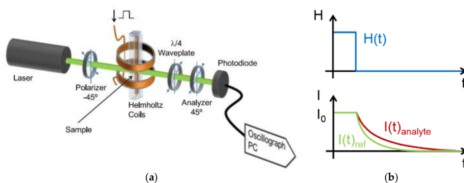
Figure 16. (a) Sketch of a typical setup for magneto-optically (Cotton-Mouton effect) measuring changes in the relaxation time of magnetic particles. Graph reproduced with permission from [262]. Copyright 2012, IOP Publishing. All rights reserved; (b) Sketch of the intensity time dependence measured by the photodiode after the magnetic field is turned off (blue curve): when the orientation of the particles relaxes, the measured intensity falls off exponentially (green curve), but with a larger time constant if analyte molecules have bound to the particle surface (red curve).
