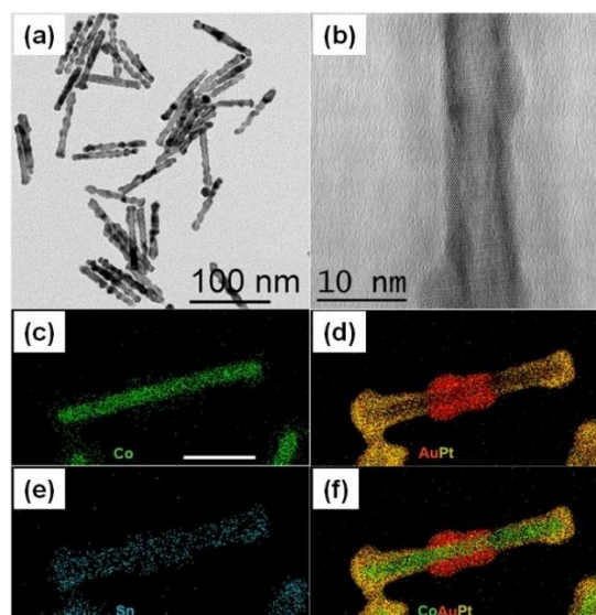
Figure 20. (a) TEM image of a Co core noble metal shell nanorod sample; (b) HRTEM image of a single nanorod, indicating a polycrystalline noble metal shell; (c)–(f) STEM-EDX elemental maps of a single nanorod to illustrate the location of the different shell elements (Co: green, Sn: blue, Au: red and Pt: yellow). The scale bar for the STEM-EDX maps is 20 nm. Reprinted with permission from [301]. Copyright 2015, American Chemical Society.
