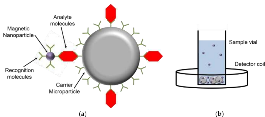
Figure 1. Schematic measurement principle of the magnetic permeability sensing method: (a) Magnetic nanoparticles (NPs) and carrier microparticles with recognition molecules on the particle surfaces bind via analyte molecules; (b) The microparticles sediment, resulting in an analyte-concentration dependent magnetic NP concentration at the bottom of the sample vial, which is placed in the center of the detection coil for determining its magnetic permeability.
