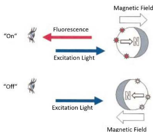
Figure 17. Sketch of modulated fluorescence by magnetic particles with a hemispherical metal coating (dark-shaded area). The coating prevents excitation/detection of fluorophores at the particle surface when the particle is rotated with the coated side towards the excitation source/observation optics by an applied magnetic field, resulting in magnetically controllable modulation of the observed fluorescence. Modified graph reprinted with permission from [218]. Copyright 2003, AIP Publishing LLC.
