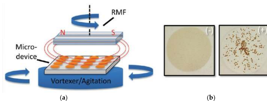
Figure 14. (a) Sketch of the dual-force setup combining a rotating magnetic field (RMF) and a vortexer to induce aggregation of magnetic particle clusters in the presence of analyte molecules; (b) The digital images show the distribution of magnetic particles within a microdevice well (well diameter 5 mm) following the agitated incubation period for a control without analyte DNA (−) and a sample with analyte DNA (+), the latter leading to agglomeration of particles visible to the naked eye. Adapted from [246] with permission of The Royal Society of Chemistry, Copyright 2015.
