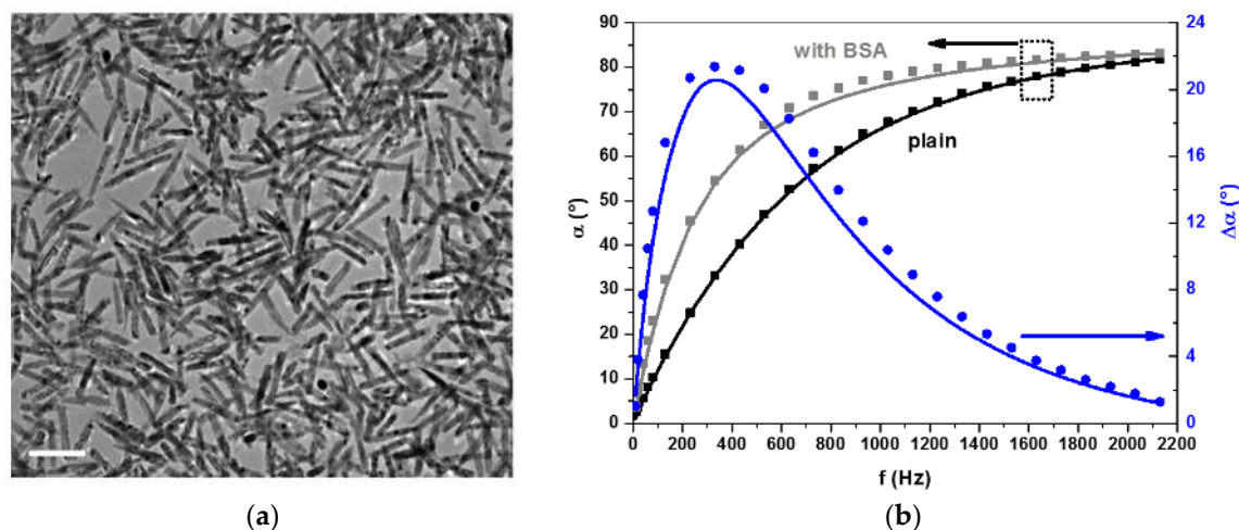
Figure 19. Ni nanorods and protein adhesion results: (a) TEM image of Ni nanorods. The scale bar corresponds to 200 nm. The mean nanorod length is 182 \pm 29 nm and the mean diameter 26 \pm 3 nm. Reprinted with permission from Reference [290]. Copyright 2014, John Wiley and Sons; (b) Phase lag \alpha spectra in dependence of the external magnetic field frequency f of Ni nanorods under addition of BSA protein and of plain nanorods at an applied RMF strength of 1 mT (left axis) and corresponding relative phase difference \Delta\alpha (right axis). Measured values (dots) are compared to the calculated model fits (lines). The relative phase difference \Delta\alpha (blue) reaches a maximum value of about 22^\circ at a frequency f of 330 Hz. Modified graph reprinted with permission from [290]. Copyright 2014, John Wiley and Sons.
