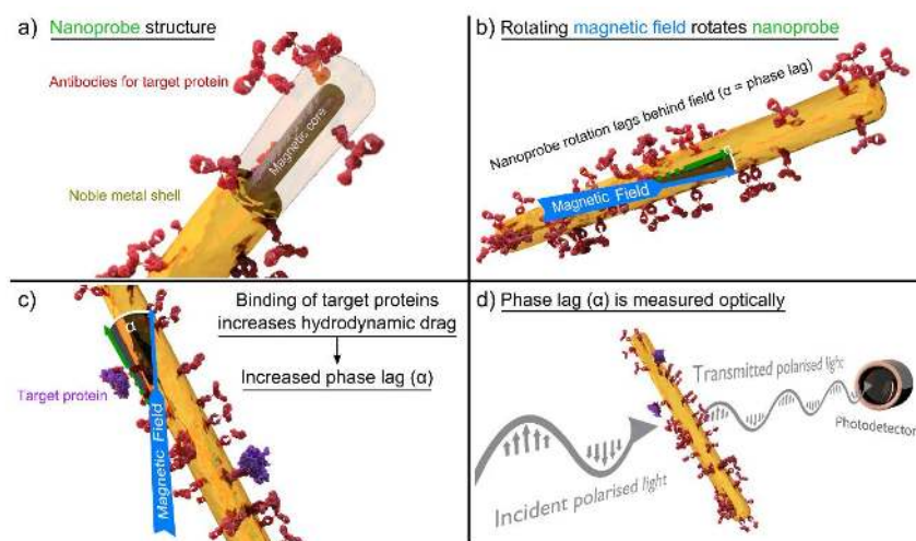
Figure 18. Sketch of the biosensing principle making use of magnetic particle labels with intrinsic optical shape anisotropy: (a) Rod-shaped nanoprobe comprising a magnetic core and a noble metal shell with antibodies on the particle surface for specific binding of target proteins; (b) The ferromagnetic nanorod follows the applied rotating magnetic field (RMF) with a phase lag \alpha due to the drag torque experienced in the sample solution, which depends on the hydrodynamic nanoprobe volume; (c) Binding of target proteins increases the hydrodynamic drag and, consequently, the phase lag \alpha ; (d) The transmission of linearly polarized light is detected. Its intensity directly relates to the actual orientation of the nanoprobe with respect to the polarization direction (angle \alpha ). Comparison of the optical signal with the momentary orientation of the RMF allows deduction of the angle \alpha . Reprinted with permission from [291]. Copyright 2016, American Chemical Society.
