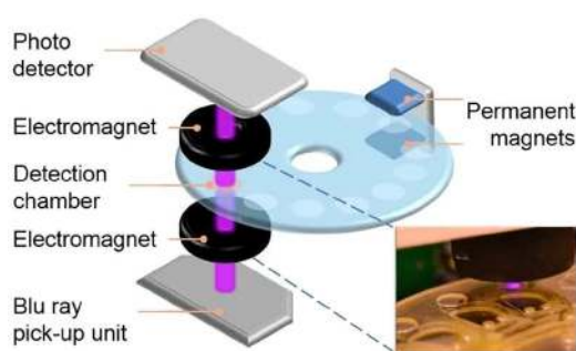
Figure 13. Sketch of the optomagnetic device incorporating Blu-ray optics introduced by Donolato et al. [239]. Reprinted with permission from [240]. Copyright 2015, Nature Publishing Group.
