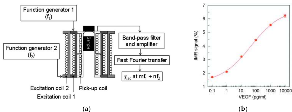
Figure 5. Schematic experimental setup and assay results of the mixed-frequency AC susceptibility measurement technique: (a) Measurement setup comprising two excitation coils and a pick-up coil for signal generation [150]. The AC susceptibility signal \chi_{AC} at mixed frequency is determined by applying read-out electronics comprising band-pass filters, a signal amplifier and Fourier transformation. Graph reprinted with permission from Hong et al. , [150]. Copyright (2007), AIP Publishing LLC; (b) Assay results and corresponding fit by the logistic function for the vascular endothelial growth factor (VEGF) protein as reported by Chieh et al. [152]. Modified graph reprinted with permission from Chieh et al. , [152]. Copyright (2010), AIP Publishing LLC.
