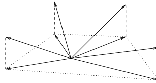
FIGURE 2. A quotient presentation of a projective toric surface
