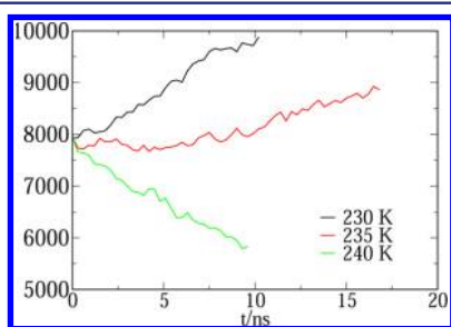
Figure 4. Number of molecules in the ice cluster versus time for system H and the TIP4P/2005 potential. Results are shown for different temperatures as indicated in the legend.
