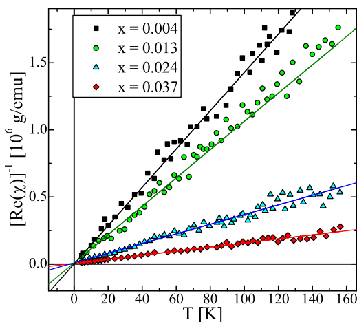
FIG. 4. The inverse of the real part of the dynamic magnetic susceptibility measured (symbols) for the selected \text{Cd}_{1-x}\text{Mn}_x\text{GeAs}_2 samples with different chemical composition. The lines represent theoretical curves fitted to Eq. (2).
