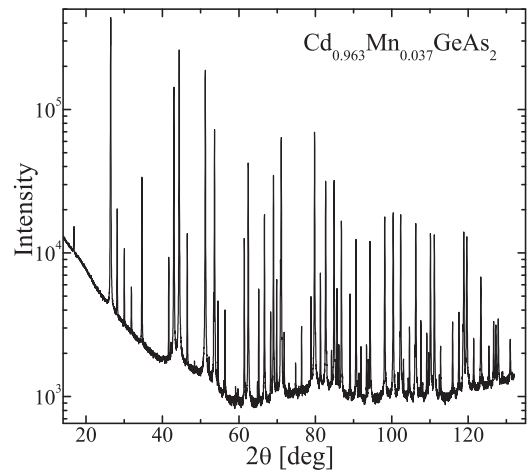
FIG. 1. Diffraction patterns observed for the exemplary Cd 1-x Mn x GeAs 2 sample with x = 0.037 .
