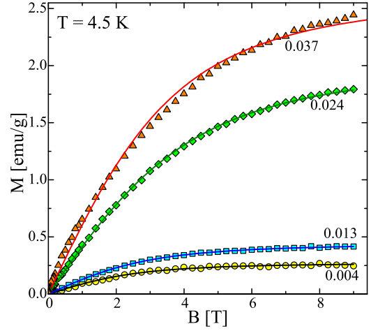
FIG. 5. The magnetization as a function of the applied magnetic field measured (symbols) at T = 4.5 \text{ K} for the selected \text{Cd}_{1-x}\text{Mn}_x\text{GeAs}_2 samples with different chemical compositions. The lines represent the theoretical curves fitted to Eq. (5).
