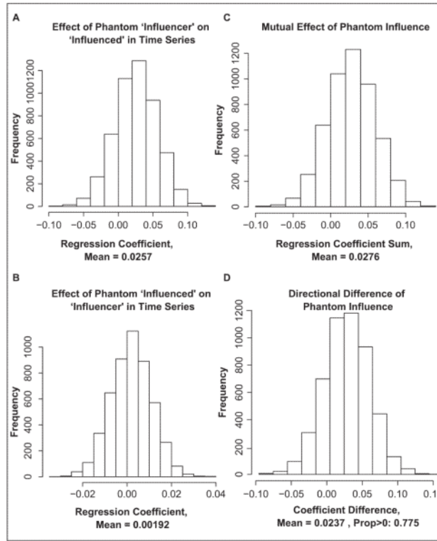
Figure 5. Results for a toy model where a latent variable causes spurious time-dependent network effects Note: Clockwise from the top left: (a) the estimate for \beta_2 , the effect in the expected direction of influence; (b) the estimate for \beta_2 , the effect in the opposite direction of influence (from the namer to the named); (c) the sum of the estimated effects, indicating that the effect for a mutual tie (in which each respondent names the other) is greater than either the expected or opposite unreciprocated tie effect; (d) the normalized difference between directional effects is clearly greater than zero on balance (in roughly 77 percent of simulations), suggesting that the asymmetry in coefficient estimates can be produced without contagion and falsely detected by t tests on the difference.
