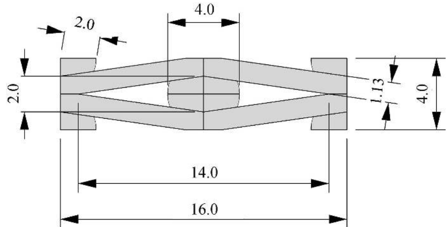
Fig 2. Swelling-honeycombs model. Diamond-shaped honeycombs inspired by the microstructure of the ice plant keel's tissue. The unit cell has a diamond shape with a width-to-height ratio of 4 for stiff walls (1.13 mm thickness) and round soft inclusions. The honeycombs were built as rectangular arrays of 5-by-10 cells. All dimensions are in mm.
