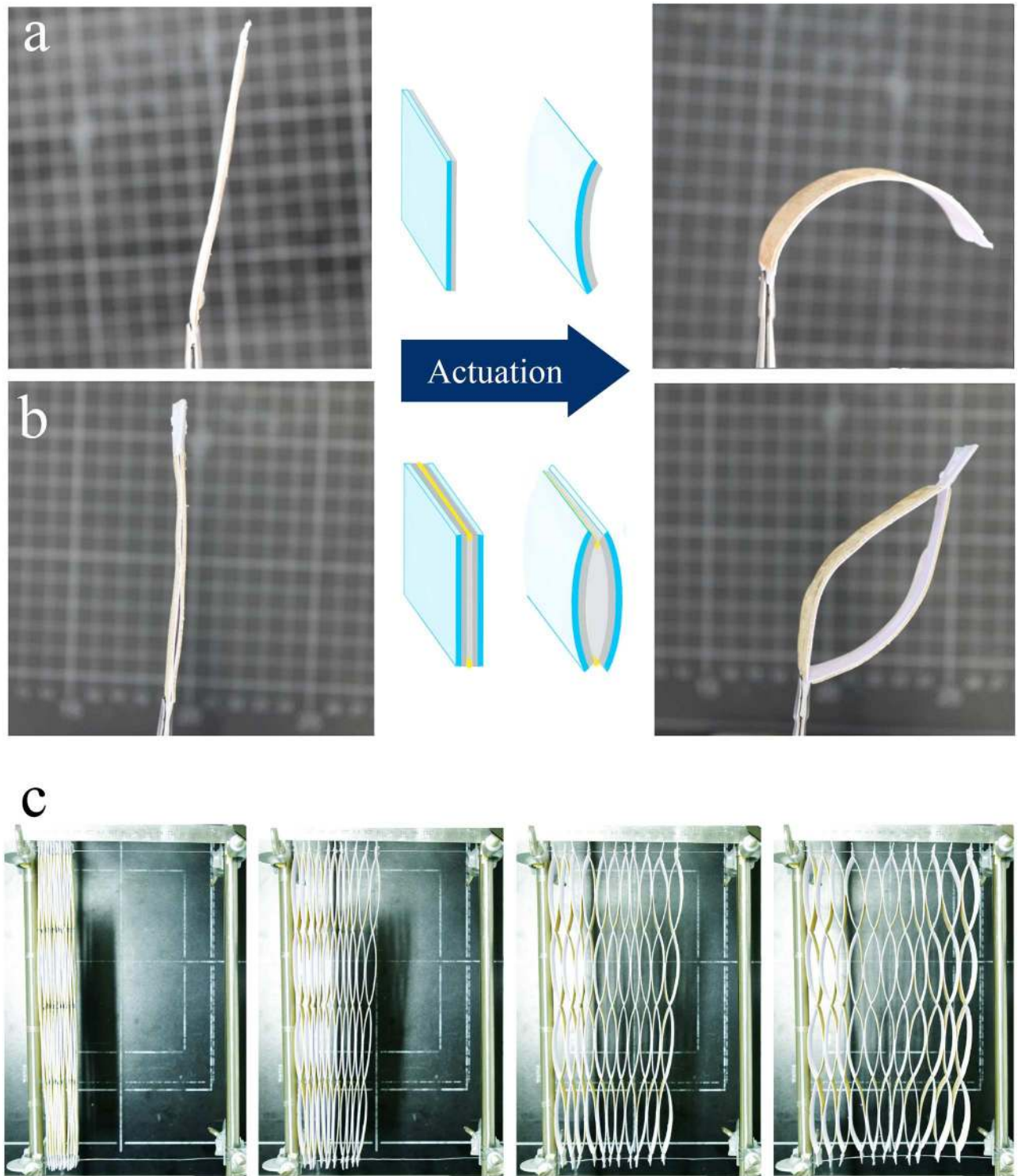
Fig 9. Passive hydro-actuation of bio-inspired bilayer-honeycomb device. Initial (left) and final actuated state (right) of the passive hydro-actuation upon changing the relative humidity from 50 to 95% are depicted at different levels of the design; (a) A bilayer made up of spruce veneer (active layer) glued to a thick paper (passive layer), bends upon anisotropic swelling of the spruce veneer in the direction perpendicular to the cellulose fibrils orientation. (b) Two of such bilayers attached together, constructs a cell-like structure that can open/closes upon changes in the relative humidity. (c) Scaling up the bilayer-cell concept into a hydro-actuated honeycomb prototype that expands up to 5 fold upon actuation (sequential images after 0, 2, 4 and 16 hours of exposure to 95%RH) [20].
