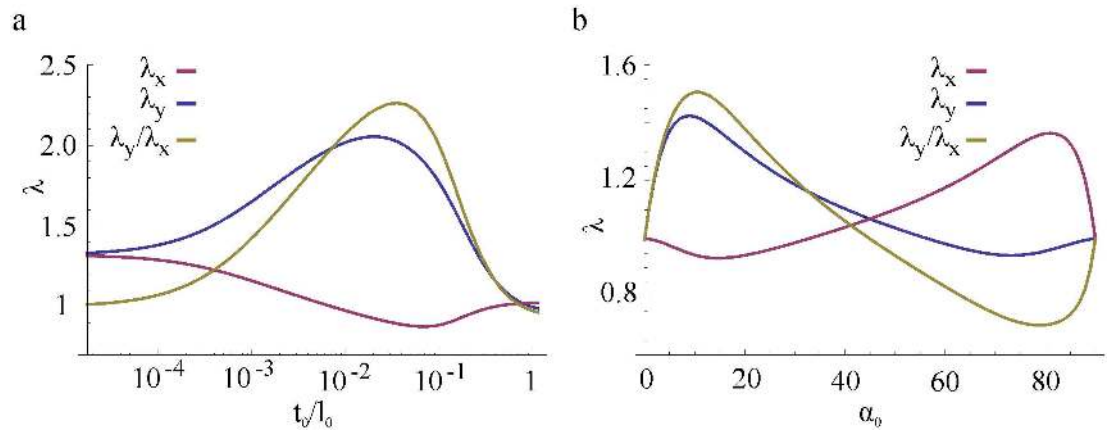
Fig 5. Influence of walls aspect ratio ( t_v/l_0 ) and honeycomb angle ( \alpha_0 ) on the honeycomb swelling deformations for G_w = G_{MW4} = 176.7 MPa and G_i = G_{MI} = 0.135 . (a) Influence of walls aspect ratio on the honeycomb expansion. For walls of vanishing thickness the honeycomb expands isotropically as the inclusions. For very thick walls the honeycomb doesn't expand at all. (b) Influence of honeycomb angle on the honeycomb expansion.
