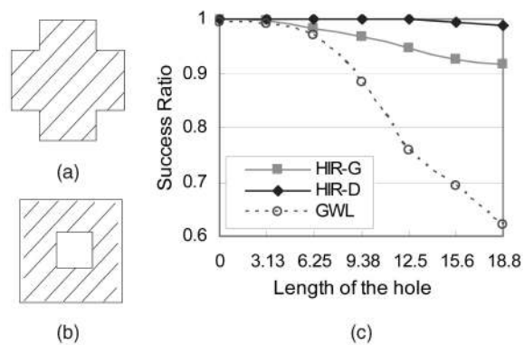
Fig. 19. Irregular shapes and success rate for shape (b) as a function of hole length.
