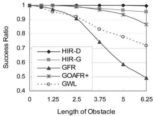
Fig. 18. Success rate as a function of obstacle length.
