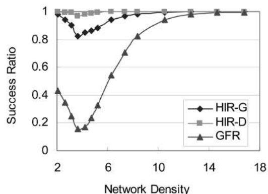
Fig. 20. Success rate as a density of density in 3D space.
