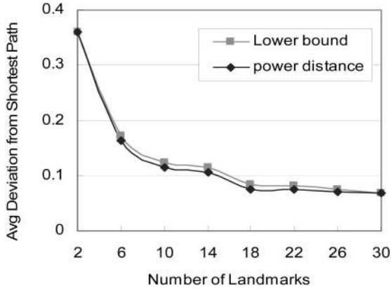
Fig. 2. Distance functions versus shortest path.
