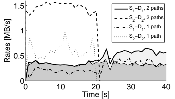
Figure 4: An example of load balancing with two flows: flows S_1 - D_1 and S_2 - D_2 (see Figure 3) compete for resources. Flow S_2 - D_2 finishes after approx 20s. The light gray area is the rate of flow S_1 - D_1 over the path shared with S_2 - D_2 , dark gray is the rate over a disjoint path.
