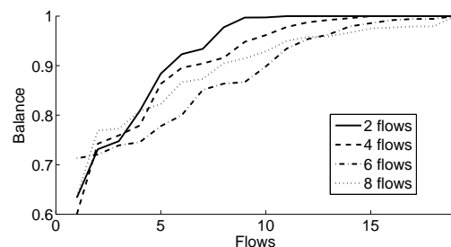
Figure 8: Fraction of the total traffic sent on one of the two paths
