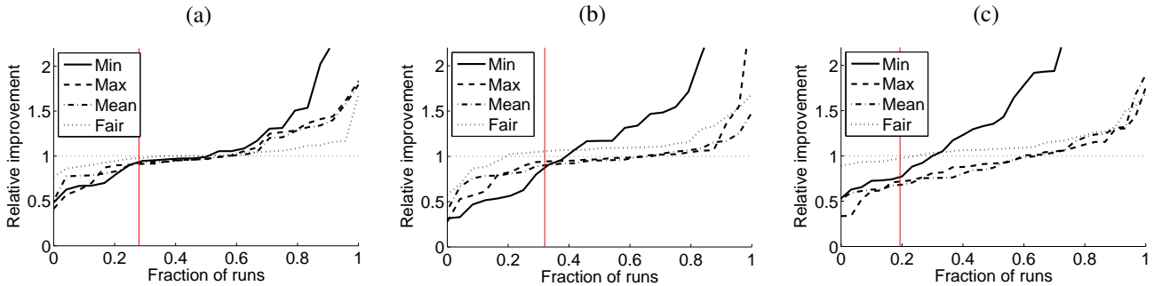
Figure 7: CDF of the relative improvement of the minimum, mean, maximum rate and the fairness index of Horizon over the single-path TCP for the experiments with 2 flows (a), 4 flows (b) and 8 flows (c). Confidence intervals are removed for clarity. Note that the points on different curves with the same x-value do not correspond to the same experiment. The experiments on the left of the vertical red line have lower utility in the case of Horizon than in the case of the single-path TCP. The experiments on the right improve the utility with Horizon .
