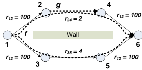
Figure 1: A network with 6 nodes. Flow f goes between nodes 1 and 6, flow g between nodes 2 and 4. Links r_{24} = 2 and r_{35} = 4 are bottlenecks and links r_{12} = r_{13} = r_{46} = r_{56} = 100 are significantly faster.
