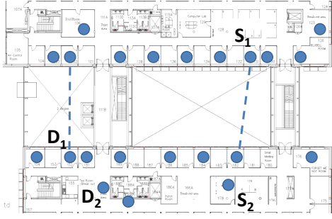
Figure 3: Floorplan of the testbed. Dots represent nodes’ locations. The area in the middle is an atrium. Only the nodes connected with dashed lines can communicate across the atrium.
