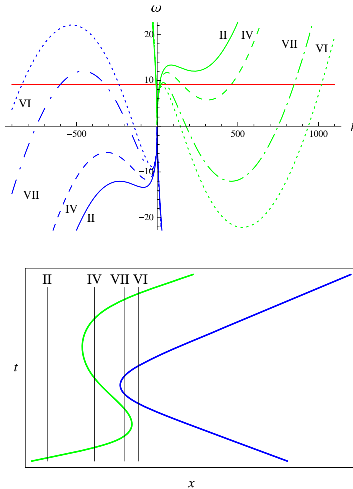
Figure 13. Dispersion plots and ray solutions for waves with period T > T_b . The Roman numerals refer to counter-flow speeds that lie in the regions labelled by these numerals in figure 7. The period is T = 0.692 s and the flow velocities are -0.192 m s ^{-1} (II), -0.214 m s ^{-1} (IV), -0.260 m s ^{-1} (VII) and -0.281 m s ^{-1} (VI).
