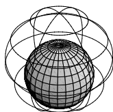
Conical horosphere.
