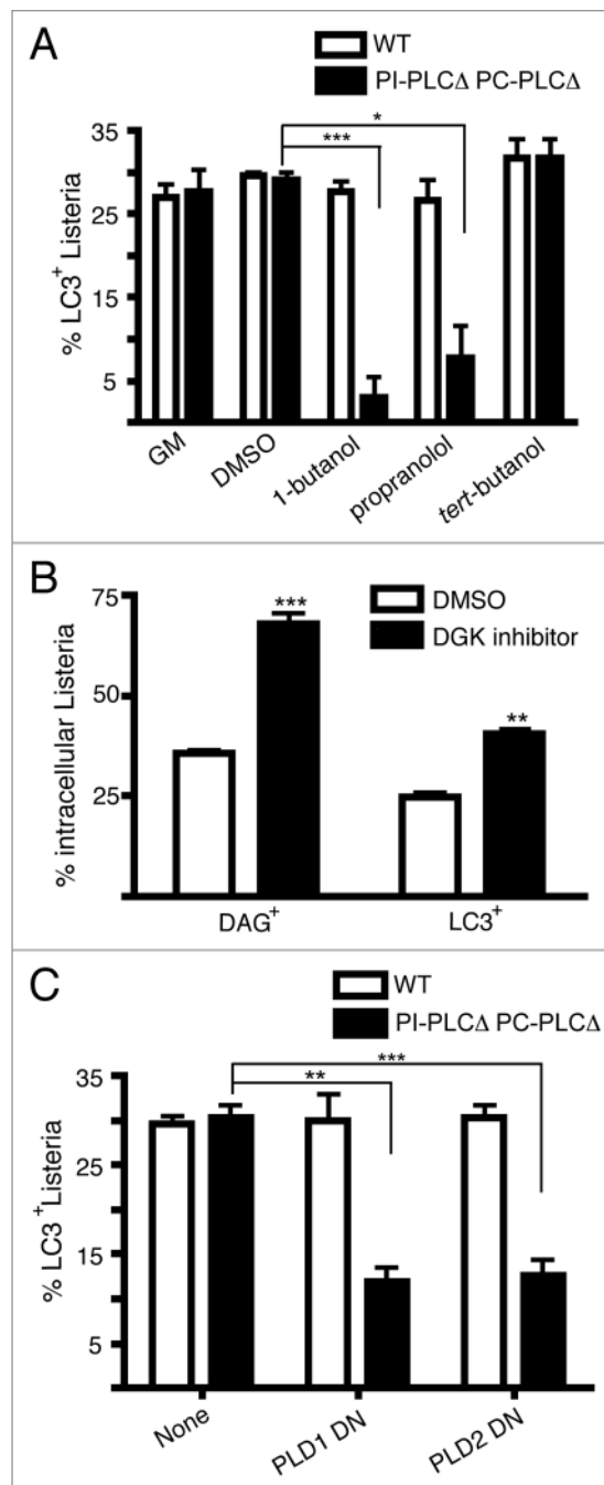
Figure 6. DAG production is required for LC3-associated phagocytosis of L. monocytogenes during early stages of infection. (A) Quantification at 1 h p.i. of intracellular wild-type or PI-PLC \Delta PC-PLC \Delta L. monocytogenes that are LC3 + following treatment with DMSO, 1-butanol, propranolol, or tert -butanol. (B) Quantification at 1 h p.i. of DAG (PRKCD-C1-GFP + ) or LC3 colocalization with wild-type L. monocytogenes with or without treatment with the DAG kinase I inhibitor. (C) Quantification at 1 h p.i. of LC3 + intracellular wild-type or PI-PLC \Delta PC-PLC \Delta L. monocytogenes in RAW 264.7 macrophages that were cotransfected with LC3-GFP and either PLD1 dominant negative (DN) or PLD2 DN constructs.
