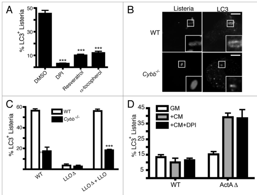
Figure 3. ROS production by the CYBB/NOX2 NADPH oxidase is required for LC3 recruitment to L. monocytogenes during early stages of infection. (A) RAW 264.7 cells were infected with wild-type L. monocytogenes for 1 h in the presence or absence of DPI, resveratrol or α-tocopherol, as indicated. The percentage of intracellular bacteria that are LC3 + upon treatment with each agent is shown. (B) Confocal images of wild-type or cybb -/- bone marrow-derived macrophages transfected with GFP-LC3 and infected for 1 h with wild-type bacteria. Size bar: 5 μm. (C) Quantification at 1 h p.i. of the percentage of intracellular L. monocytogenes that are LC3 + in bone marrow-derived macrophages isolated from wild-type or cybb -/- mice. Wild-type bacteria were compared with LLOΔ bacteria (negative control), as well as a LLOΔ mutant complemented with LLO. (D) Quantification of the percentage of L. monocytogenes that are LC3 + in RAW 264.7 macrophages infected with either wild-type or ActAΔ bacteria for: 8 h (GM); 3 h, followed by 5 h Cm treatment (+Cm); or 3 h, followed by 5 h Cm and DPI treatment (+Cm +DPI).
