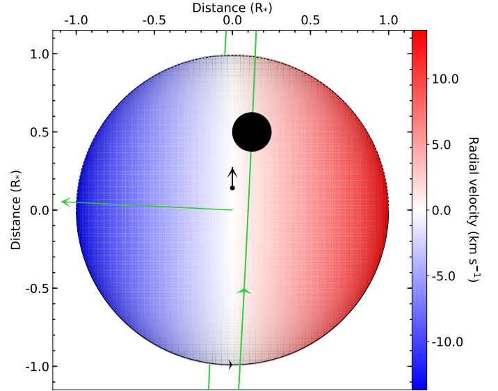
Fig. 10. Projection of WASP-121 in the plane of sky for the best-fit scenario where the north pole of the star is visible. The stellar spin axis is displayed as a black arrow extending from the north pole. The stellar equator is represented as a black line, solid when visible and dashed when hidden from view. The stellar disk is colored as a function of its RV field. The normal to the orbital plane is shown as a green arrow, and the orbital trajectory is displayed as a green curve. The black disk is WASP-121b, to scale.
