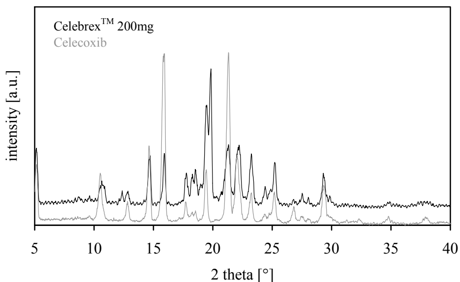
Figure 4.82: XRPD pattern of original product Celebrex TM and the drug CEL
