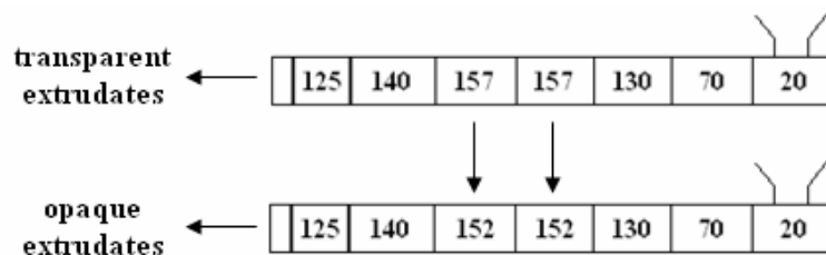
Figure 4.7: Temperature profiles of the extruder barrel for the production of transparent and opaque strands of CEL/aPMMA 1:1 (w/w)
