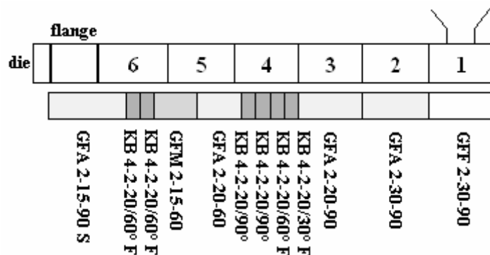
Figure 4.1: Extruder barrel, configuration of the screw, and position of the screw elements; GFF & GFA = conveying elements, GFM = combing mixer element, KB = kneading block
