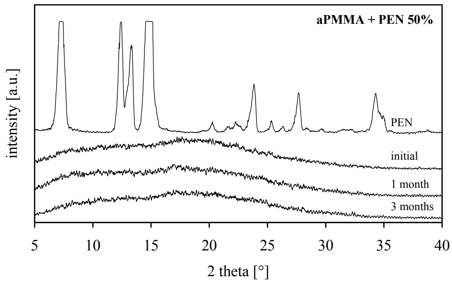
Figure 8.19: Stability of aPMMA/pentoxyfylline 1:1 (w/w) extrudates at 25 °C over silica gel
