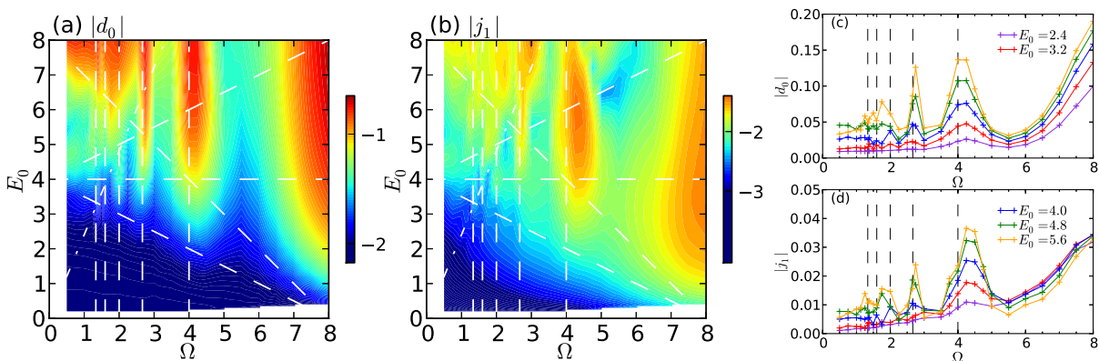
FIG. 6. (a,b) Log scale plot of the static components of the double occupancy (time-averaged, |d_0| ) and the 1st order harmonic component of the current ( |j_1| ) in the plane of the field strength E_0 and the excitation frequency \Omega . (c)(d) Cuts for fixed E_0 . Here, U = 8.0 , \beta = 2.0 , \Gamma = 0.06 , W_{\text{bath}} = 5.0 .
