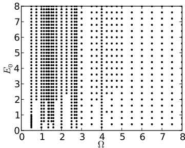
FIG. 15. Data points used for Fig. 6 and Fig. 10.
