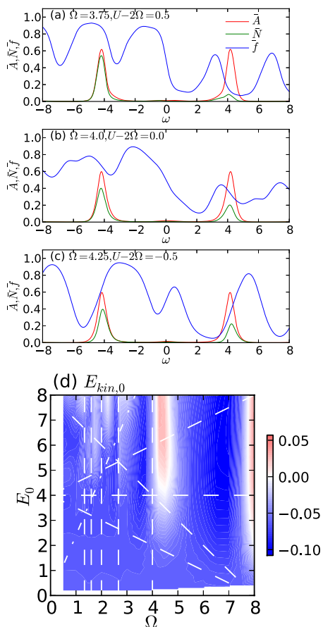
FIG. 5. (a-c) Time-averaged local spectrum, occupation and distribution function around \Omega = U/2 . The field strength is E_0/\Omega = 1.841 . (d) Time-averaged kinetic energy in the plane of E_0 and \Omega . Here, U = 8.0, \beta = 2.0, \Gamma = 0.06, W_{\text{bath}} = 5.0 .
