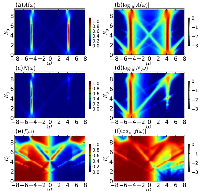
FIG. 2. (a)(b) The local spectral function A(\omega) , (c)(d) the occupation function N(\omega) and (e)(f) the distribution function f(\omega) of the Hubbard model with DC field. The parameters are U = 8.0 , \beta = 2.0 , \Gamma = 0.06 , W_{\text{bath}} = 5.0 .
