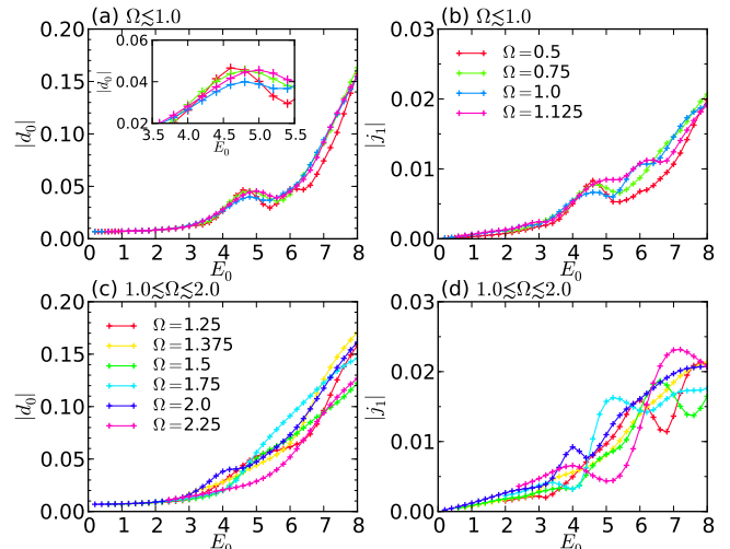
FIG. 7. E_0 -dependence of d_0 and j_1 in the small- \Omega regime. Here, U = 8.0 , \beta = 2.0 , \Gamma = 0.06 , W_{\text{bath}} = 5.0 .
