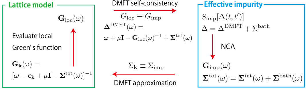
FIG. 1. FDMFT self-consistency loop. Boldfied letters indicate the Floquet representation of the corresponding function. S_{\text{imp}} is the impurity action, which is determined by the hybridization function. In the present case, the hybridization function consists of the effective bath which mimics the surrounding lattice ( \Delta^{\text{DMFT}} ), and the attached electron bath ( \Sigma^{\text{bath}} ). The problem is solved by NCA which yields the impurity Green's function and the self-energy ( \Sigma^{\text{tot}} ) consisting of the contribution from the interaction ( \Sigma^{\text{int}} ) and that from the bath ( \Sigma^{\text{bath}} ). Using this and \epsilon_{\mathbf{k}}(t) = \epsilon(\mathbf{k} - \mathbf{A}(t)) we obtain the lattice Green's function at each momentum, and by averaging over \mathbf{k} the local Green's function. Through the impurity Dyson equation we update the hybridization function.
