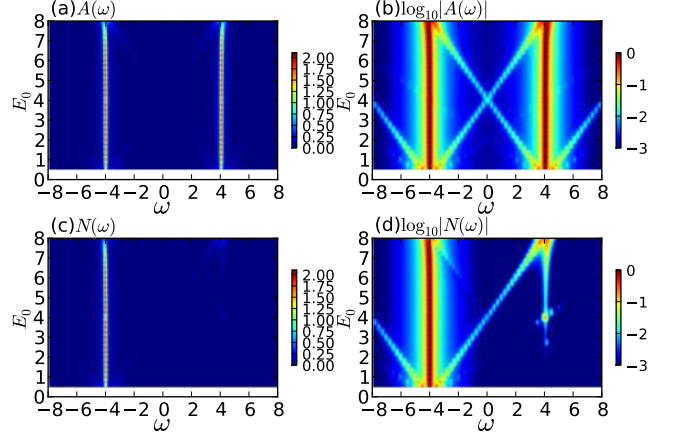
FIG. 13. (a)(b) Local spectral function ( A(\omega) ) and (c)(d) occupation function ( N(\omega) ) of the semiconductor model with a DC field. Here, U = 8.0, \beta = 2.0, \Gamma = 0.06 .
