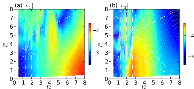
FIG. 10. (a)(b) Log-scale plot of the linear ( |\sigma_1| ) and third harmonic ( |\sigma_3| ) conductivity. Here, U = 8.0, \beta = 2.0, \Gamma = 0.06, W_{\text{bath}} = 5.0 .
