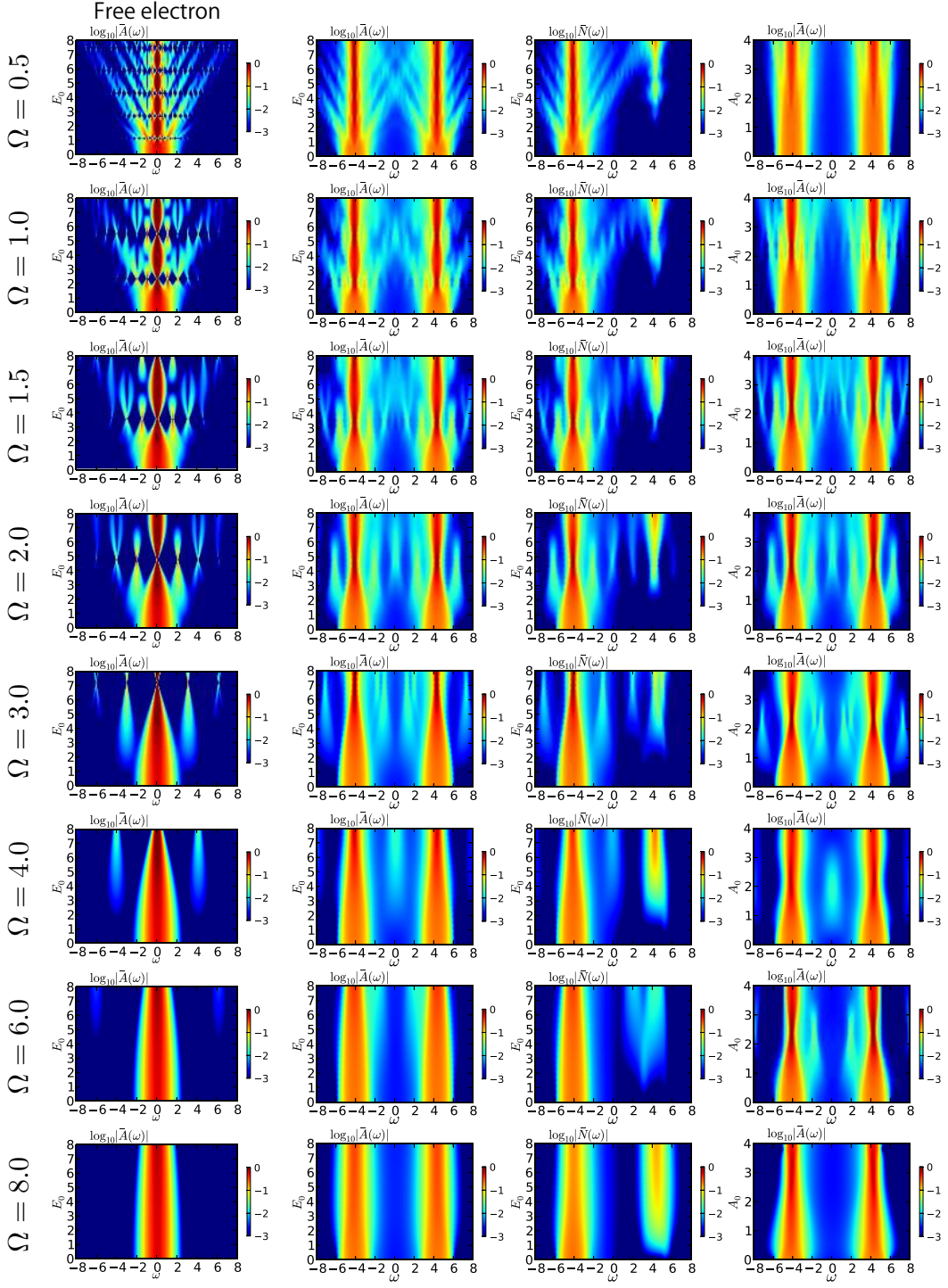
FIG. 4. Log scale plots of the local spectral function \bar{A}(\omega) and occupation function \bar{N}(\omega) of the Hubbard model driven by AC fields with indicated frequencies \Omega and amplitudes E_0 . Here, U = 8.0, \beta = 2.0, \Gamma = 0.06, W_{\text{bath}} = 5.0 .
