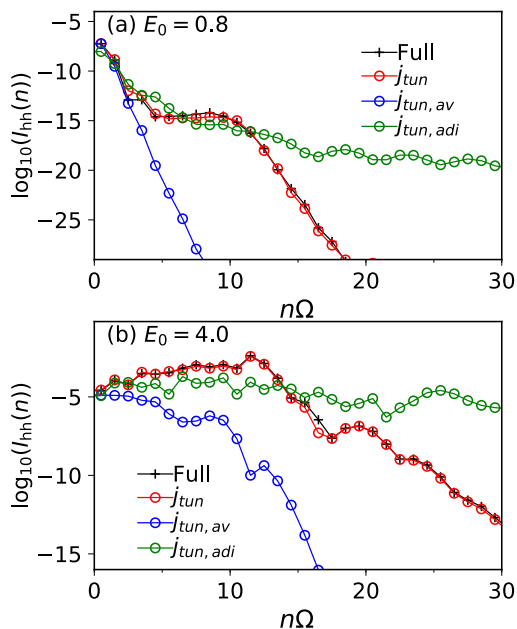
FIG. 11. Comparison of the high-harmonic generation spectra evaluated by different tunneling formulas. Here, U = 8.0 , \beta = 2.0 , \Gamma = 0.06 , W_{\text{bath}} = 5.0 .
