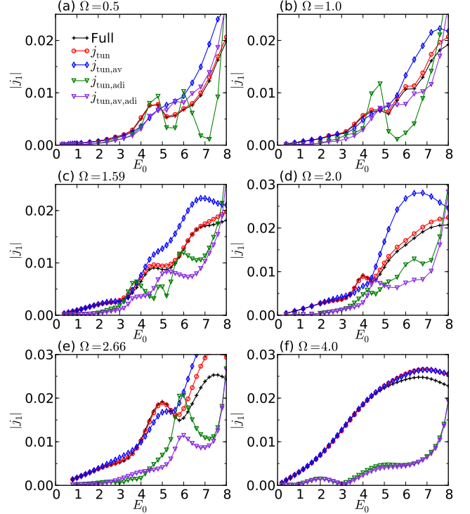
FIG. 9. Comparison of |j_1| evaluated by different tunneling formulas for selected excitation frequencies near the resonances n\Omega = U . Here, U = 8.0, \beta = 2.0, \Gamma = 0.06, W_{\text{bath}} = 5.0 .
