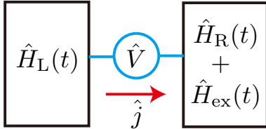
FIG. 12. Schematic picture of two subsystems in Floquet steady states, which are connected by junctions ( \hat{V} ).
