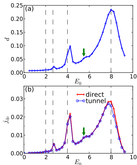
FIG. 3. (a)(b) Field-strength dependence of the double occupancy ( d ) and the current ( j_{\text{dc}} ) of the Hubbard model with DC field. In panel (b), the measured current is shown with red cross marks, while the current estimated by the tunneling formula, Eq. (14), is shown with blue circles. Vertical lines indicate E_0 = U, U/2, U/3 , and U/4 , and the arrows indicate humps at E_0 \simeq 5.5 \simeq \frac{2}{3}U . Here, U = 8.0 , \beta = 2.0 , \Gamma = 0.06 , W_{\text{bath}} = 5.0 .
