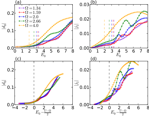
FIG. 8. E_0 -dependence of d_0 and j_1 near the resonances \Omega = U/n . Panels (a)(b) show the original data, and panels (c)(d) the results with the horizontal axis shifted by the “threshold field” E_{0,\text{line}} = (U - \Omega)/2 . Vertical lines indicate E_{0,\text{line}} for the parameters specified by the colors. Here, U = 8.0, \beta = 2.0, \Gamma = 0.06, W_{\text{bath}} = 5.0 .
