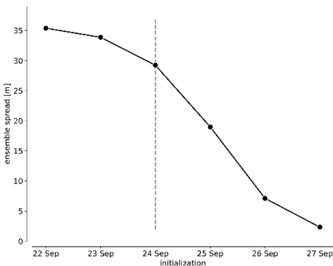
Figure 5. Area-averaged ensemble spread of geopotential height at 500 hPa at 00:00 UTC 27 September 2018 in a box over the Mediterranean ( 30\text{--}45^\circ\ \text{N} , 5\text{--}30^\circ\ \text{E} ; see black box in Fig. 7) for initializations at 00:00 UTC 22 to 27 September 2018 (black dots and line). The initialization used in this study (00:00 UTC 24 September 2018) is indicated by the dashed line.
