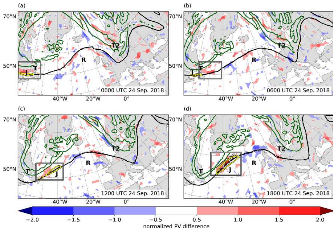
Figure 9. Normalized PV differences between clusters E and W ( \Delta PV_{EW} , shaded), 2 PVU contour (black lines) of clusters E (solid) and W (dashed), 9 PVU contour (green lines) and wind speed (yellow lines, 70 \text{ m s}^{-1} ) in the operational analysis at 325 K from 00:00 UTC 24 September to 18:00 UTC 24 September 2018, every 6 h. Regions with statistically significant PV differences ( \alpha_{fdr} < 0.1 , single isolated significant grid points are removed) are marked with white contours, and grey boxes mark the regions of interest (for details see text).
