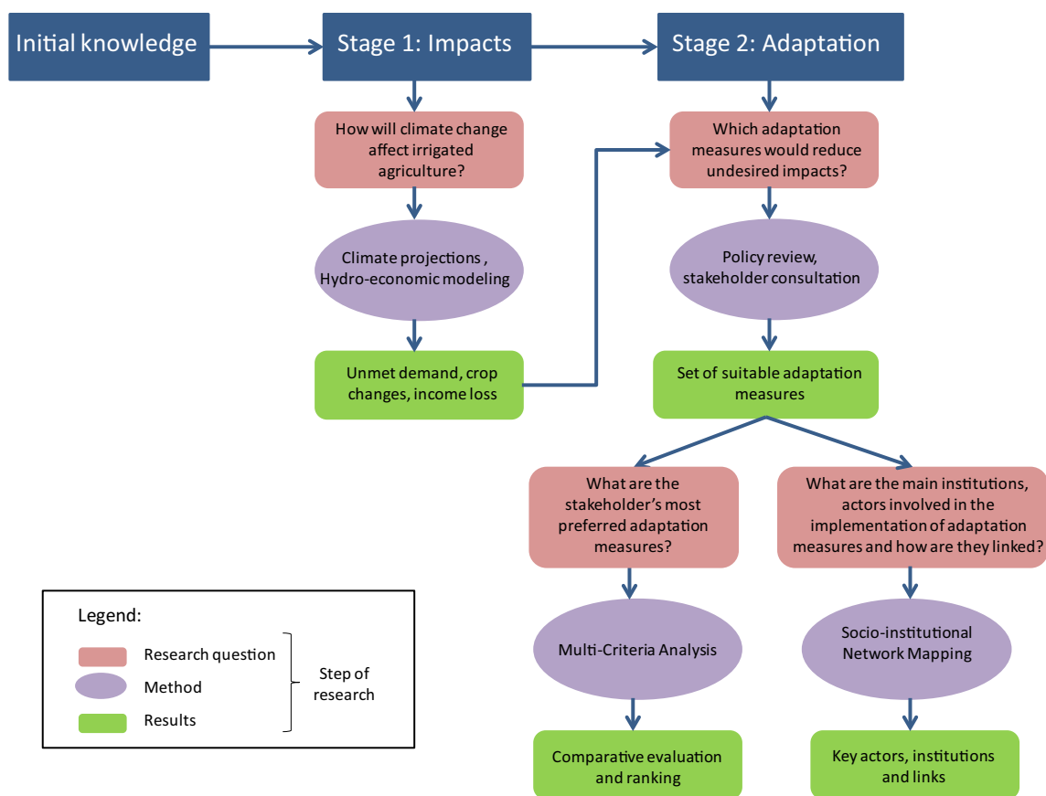
Fig. 1 Application of the diagnostic framework to analyze climate change adaptation for water and agriculture in the Guadiana Basin
