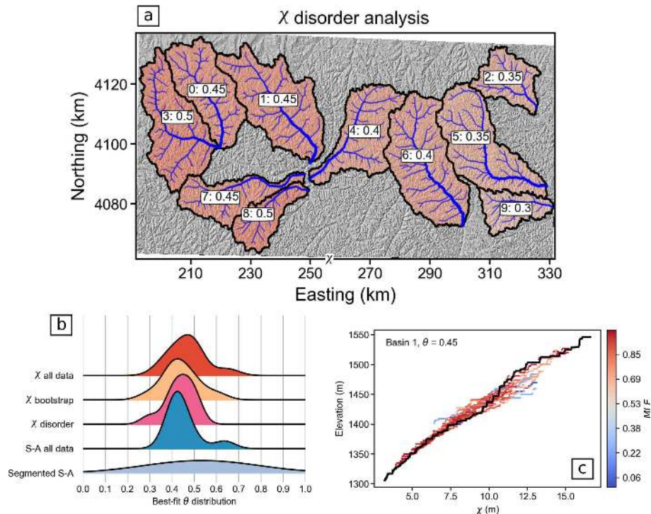
Figure 9. Exploration of the most likely concavity indices in the Loess Plateau, China, Universal Transverse Mercator (UTM) zone 49N. Basins with the most likely concavity index determined by the disorder method are displayed in panel (a); the basin number is followed by the most likely concavity index in the basin labels. The probability density of best-fit concavity index for all the basins (i.e. not the uncertainty within individual basins but rather the probability distribution of the best-fit concavity indices of all the basins) is displayed in panel (b). In basin 1, the most likely concavity index determined by the bootstrap and disorder methods is 0.45 and the \chi -elevation plot for this concavity index is shown in panel (c).
