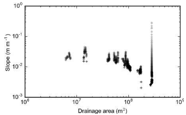
Figure 2. A typical slope–area plot. This example is from a basin near Xi’an, China, with an outlet at approximately 34°26′23.9″ N, 109°23′13.4″ E. The data are taken from only the trunk channel. The slope–area data typically contain gaps due to tributary junctions, as well as wide ranges in slope for the reaches between junctions due to topographic noise inherent in deriving slope values. The result is a high degree of scatter in the data. These data are produced by averaging slope values over a fixed vertical interval of 20 m.
