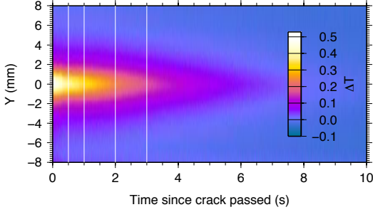
Figure 5. Space time diagram of the experimentally observed temperature increase behind the tip, as function of the y -coordinate, with respect to the position of the tip when it passed along this profile, and the time elapsed since the tip crossed the profile.
