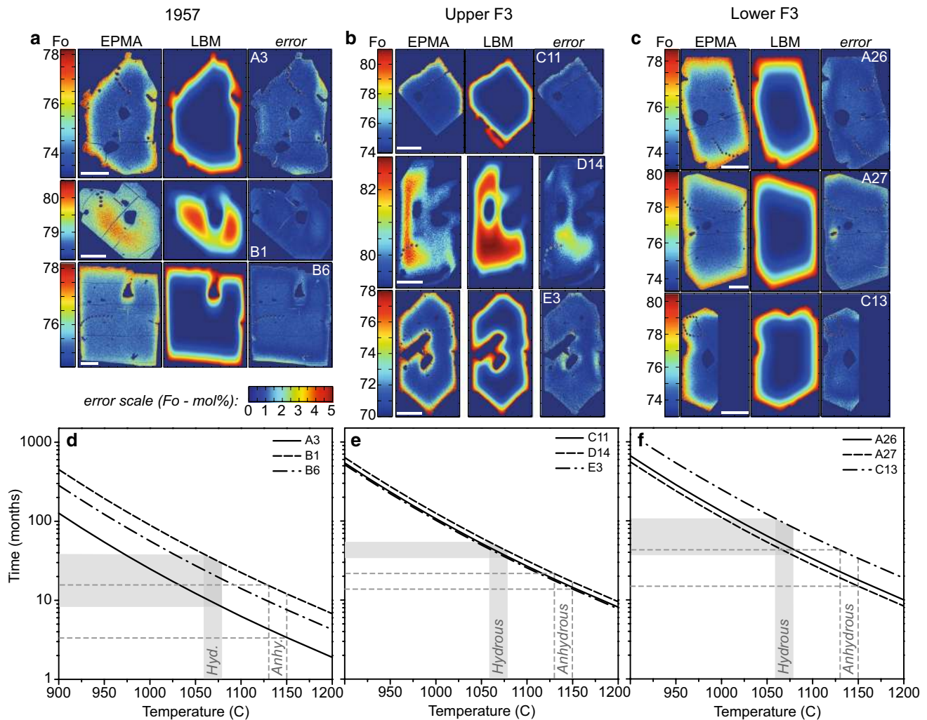
Fig. 7 2D lattice Boltzmann modeling (LBM) of the Fo zoning in the nine olivine crystals studied from the 1957 ( a , d ), UF3 ( b , e ), and LF3 ( c , f ) tephra deposits. ( a – c ) EPMA Mg X-ray maps converted to quantitative Fo maps, best fit Fo zoning map from LBM, and spatial distribution of the error (here shown as the difference in concentration between modeled and measured Fo) are shown for all crystals.
