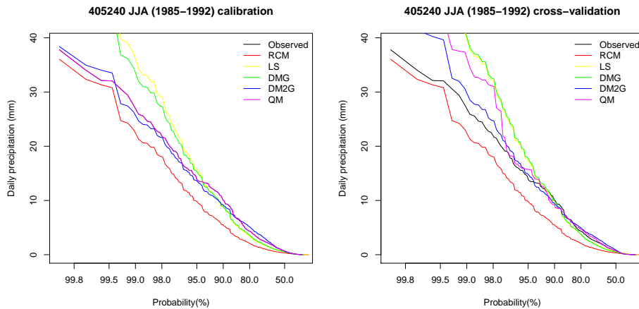
Figure 11. Comparison of CDFs derived from observed, raw RCM and bias-corrected RCM daily precipitation data for one study catchment. The left plot shows calibration results (note that the observed precipitation is completely hidden by QM in this plot) and the right plot shows cross-validation results.
