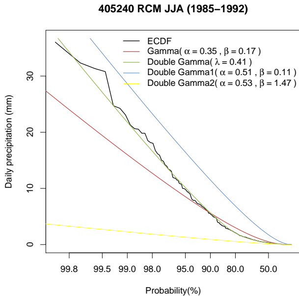
Figure 2. CDF plot comparing a gamma distribution (red) and a double gamma distribution (green), which consists of two gamma distributions (blue and yellow) fitted to the same precipitation data for one study catchment. The empirical distribution is shown in black.
