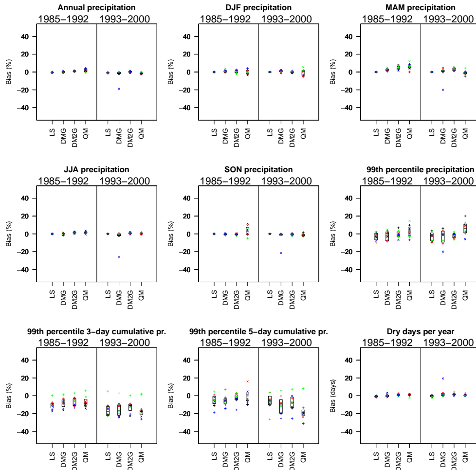
Figure 7. Differences between bias-corrected RCM and raw RCM simulations in change signals in precipitation characteristics between the periods 1985–1992 and 1993–2000. The left and right panels indicate the validation periods in each case.
