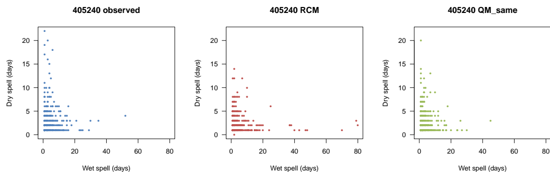
Figure 13. Scatter plots showing the length of each dry spell on y axes and the length of the following wet spell on x axes for observed, raw RCM and QM bias-corrected RCM precipitation for an example catchment.
