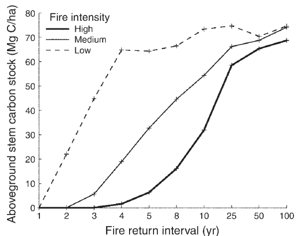
FIG. 8. Modeled aboveground tree carbon stock for the three fire intensity classes and a range of return intervals.
