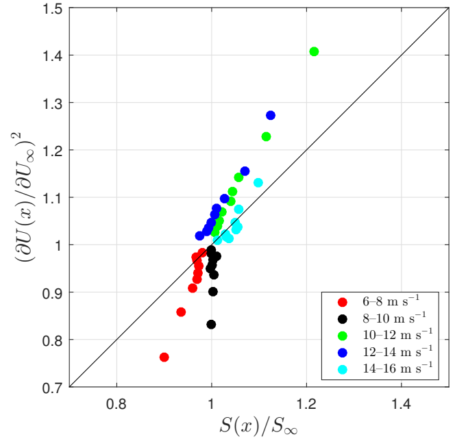
Figure 5. Change in low-frequency ( f < 0.007 \text{ Hz} ) spectral power of the longitudinal velocity component measured by the lidar compared to (\partial U(x)/\partial U_\infty)^2 . The different points for a given wind speed interval correspond to different distances from the rotor x .
